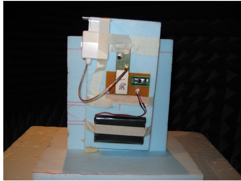
Radiated - Below 1 GHz Pifa antenna - position X
