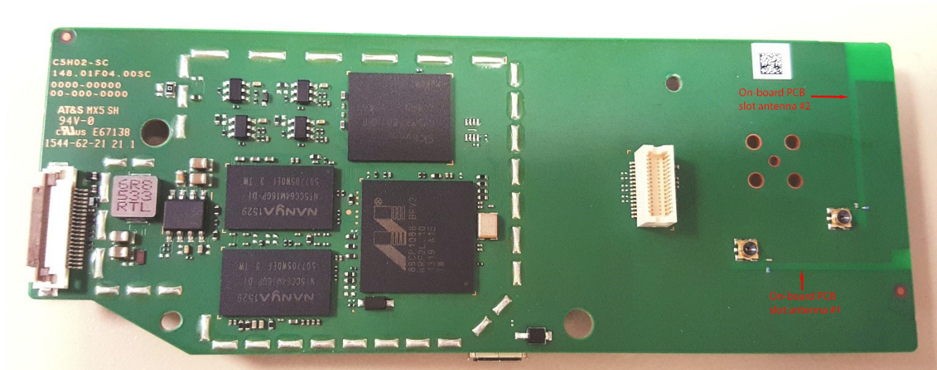
Circuit Board – Side 2 with Shield Removed
