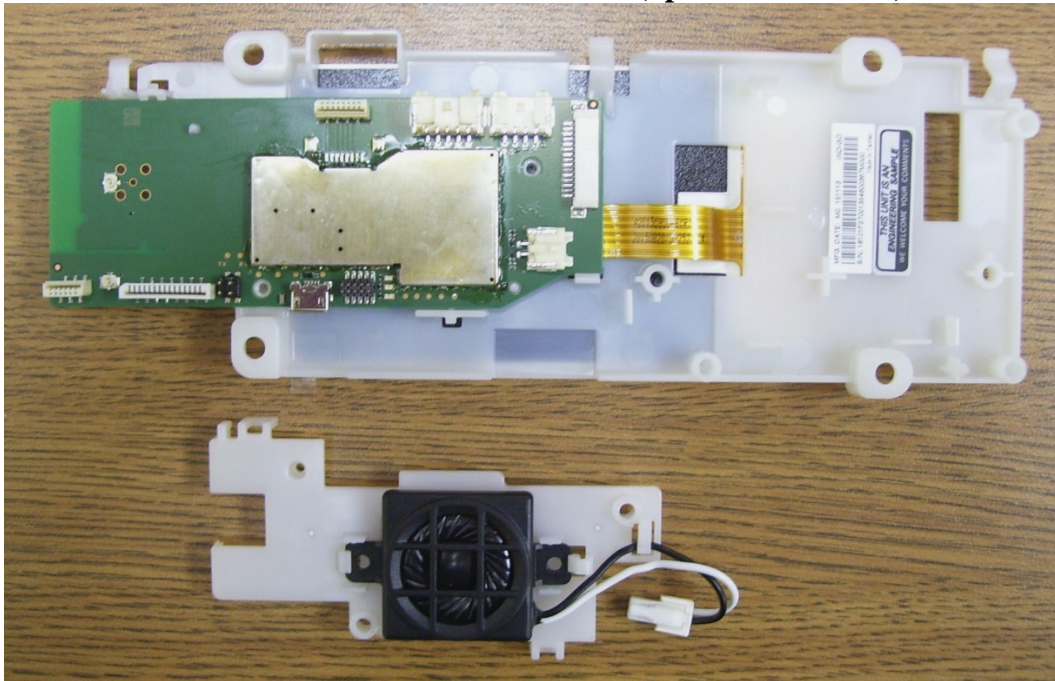
Circuit Board – Side 1 with Shield (Speaker Removed)
