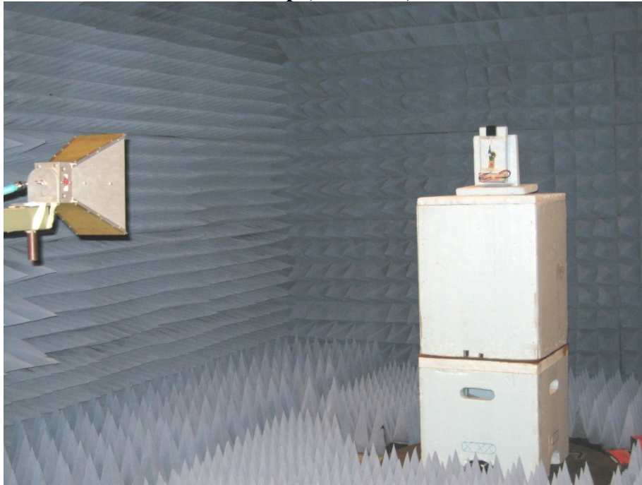
Set-up (Position 2)
