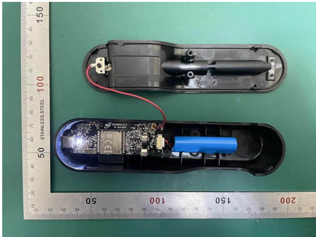
Repeater
