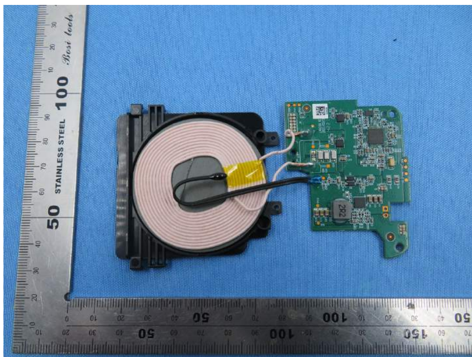
Picture 3. Front view of PCB (LXA209)
