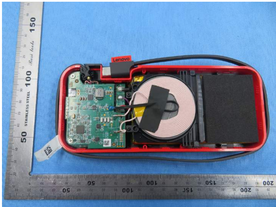
Picture 1. Internal view-1 of Power Bank
