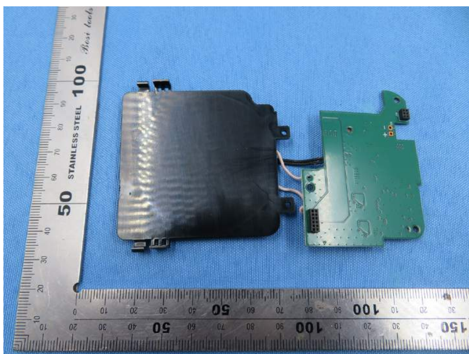
Picture 4. Rear view of PCB (LXA209)
