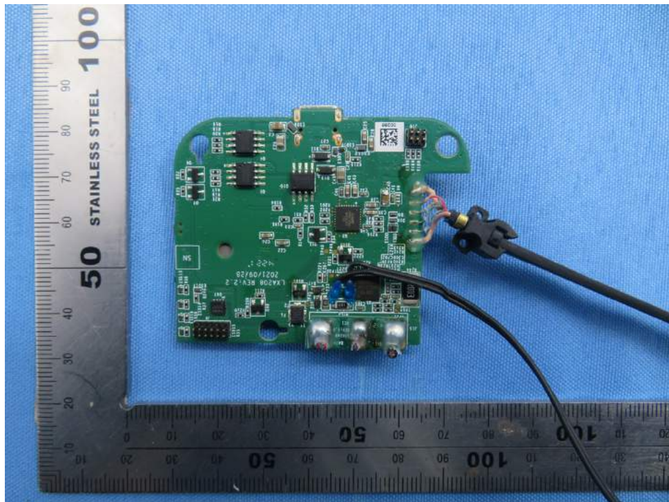
Picture 5. Front view of PCB (LXA208)
