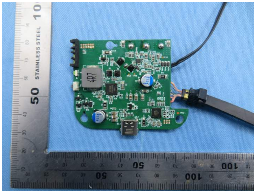
Picture 6. Rear view of PCB (LXA208)
