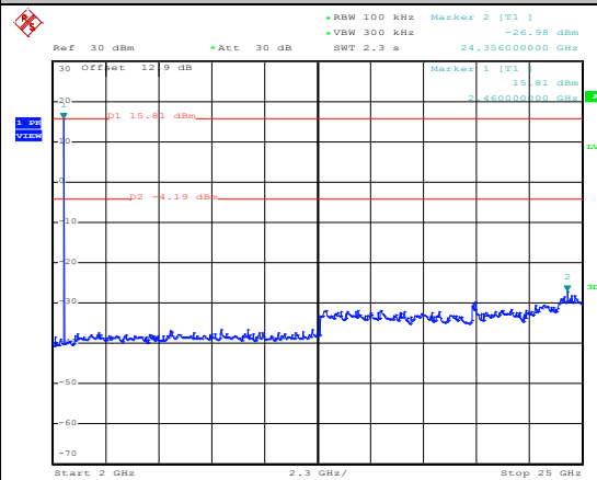
CSE Plot on CH 78 between 2 GHz ~ 25 GHz
