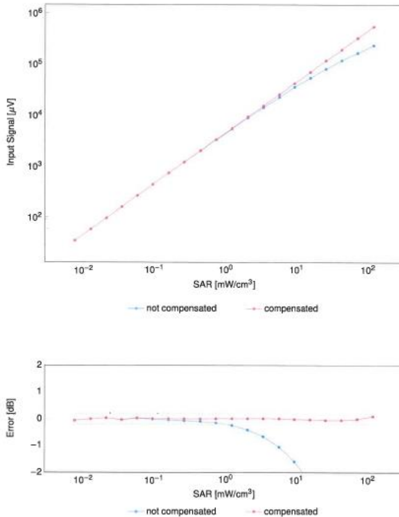
Dynamic Range f(\text{SAR}_{\text{head}}) (TEM cell, f_{\text{eval}} = 1900 \text{ MHz} )
