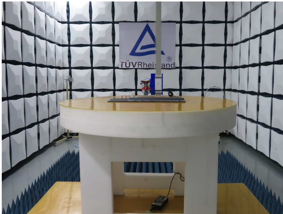
Photograph 3: Set-up photo for Radiated Spurious Emission, above 1GHz
