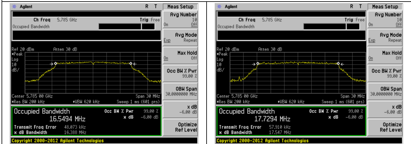
Middle channel
