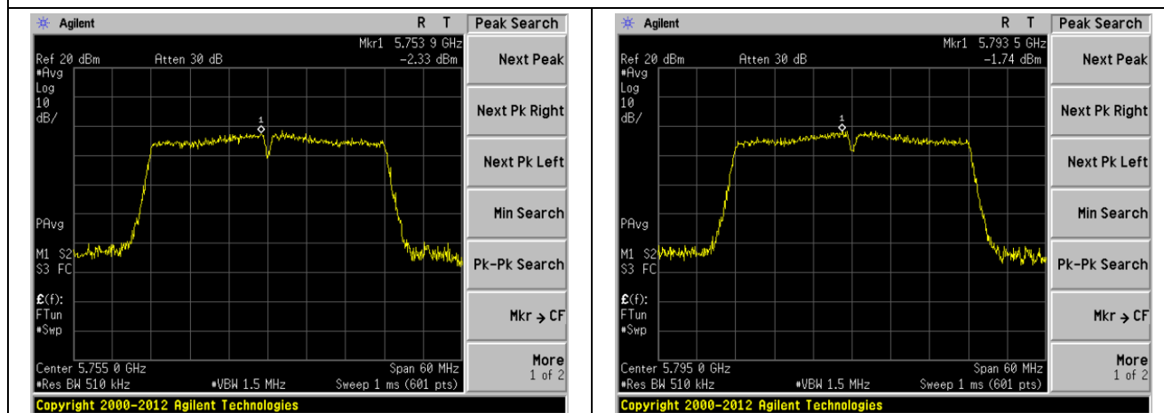
Highest channel
