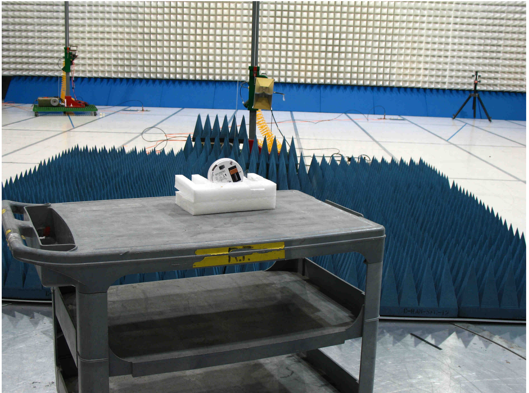
Test Setup (Back)
