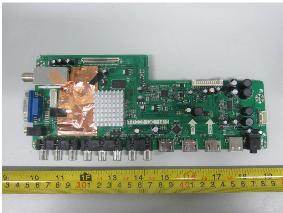
EUT – Signal Board Top View
