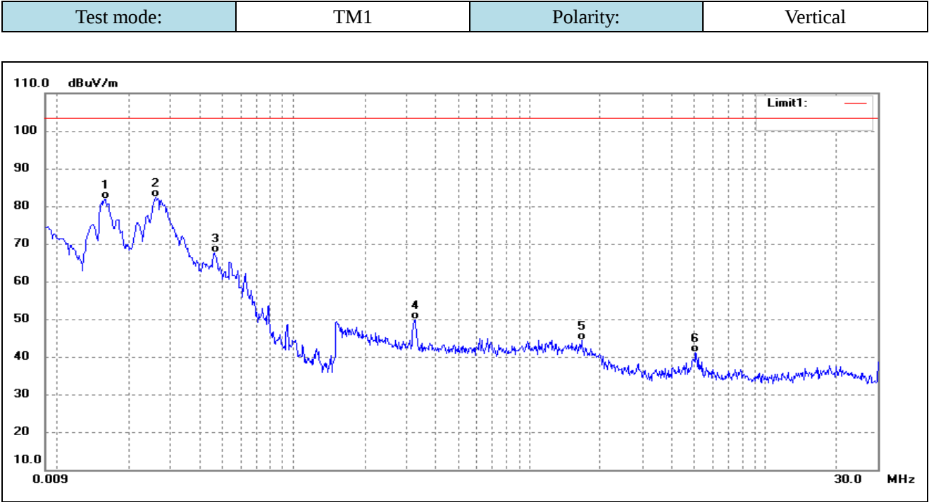
Plot of Radiated Emissions Test Data (Below 30MHz)
