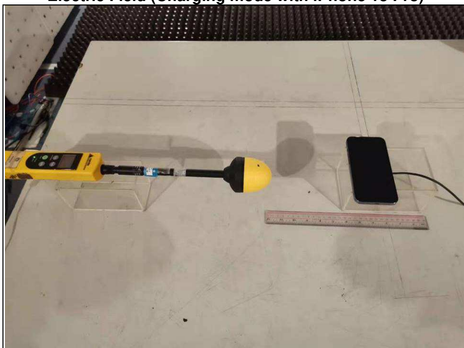
Electric Field (Charging mode with iPhone 13 Pro)
