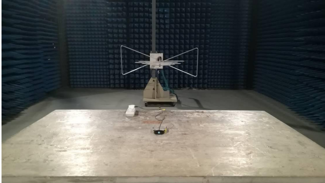
Radiated Emission
