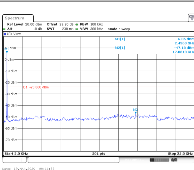
Spurious Emission 2GHz~25GHz
