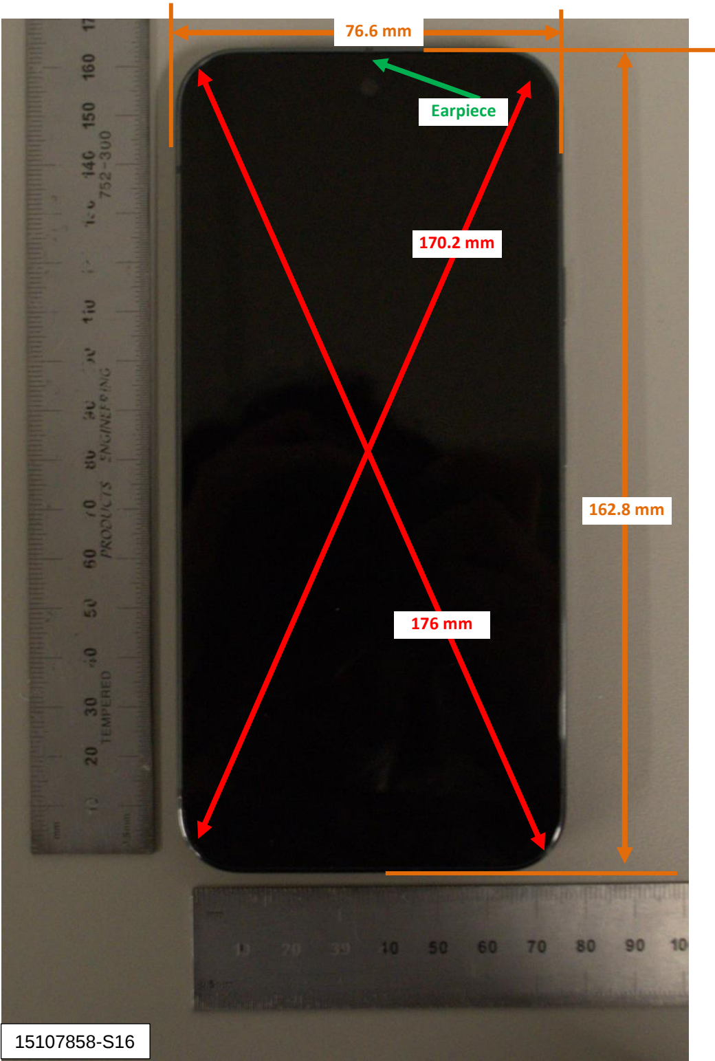
Photograph 1: Overall Dimensions
