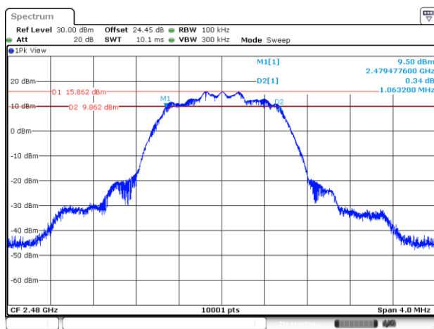
6 dB Bandwidth Plot on Channel 78
