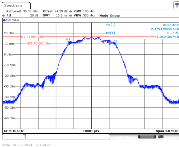
6 dB Bandwidth Plot on Channel 78
