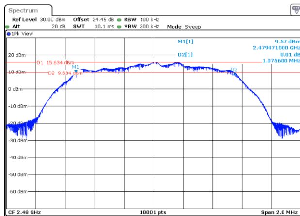
6 dB Bandwidth Plot on Channel 78
