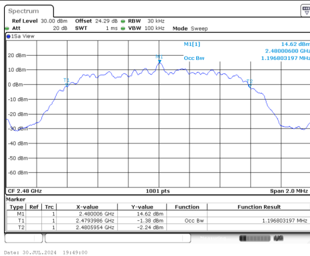
99% Occupied Bandwidth Plot on Channel 78
