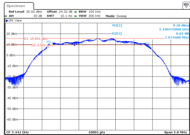
6 dB Bandwidth Plot on Channel 39
