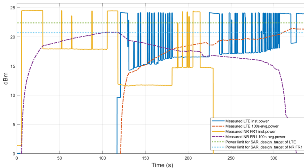
Figure 6.7-1 Time average SAR of LTE B66 and FR1 n41 in EN-DC case
