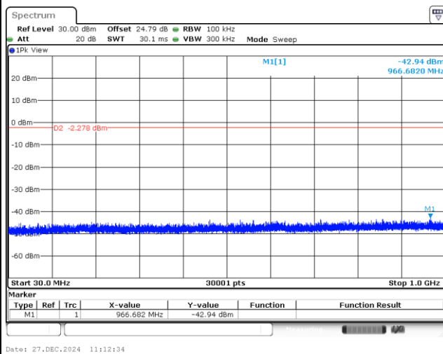
CSE Plot on Middle Ch between 30MHz ~ 1 GHz
