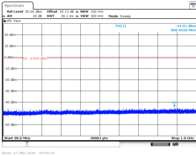
CSE Plot on Middle Ch between 30MHz ~ 1 GHz
