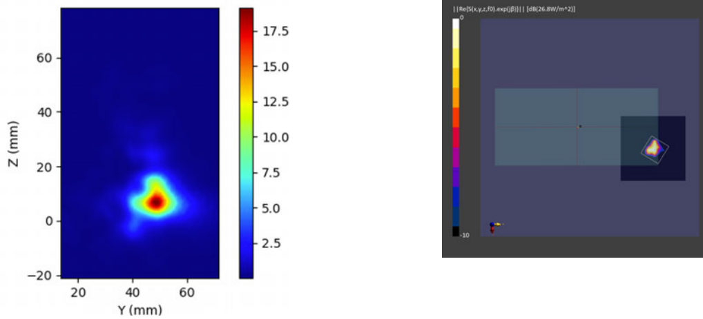
Figure 2-8 Simulated (left) and measured (right) PD distribution for the following configuration: Band n258, MID Channel, Beam ID 4, H polarization, Plane B Module, plotted on the surface S2 (back) with 2mm separation distance to the camera bump.
