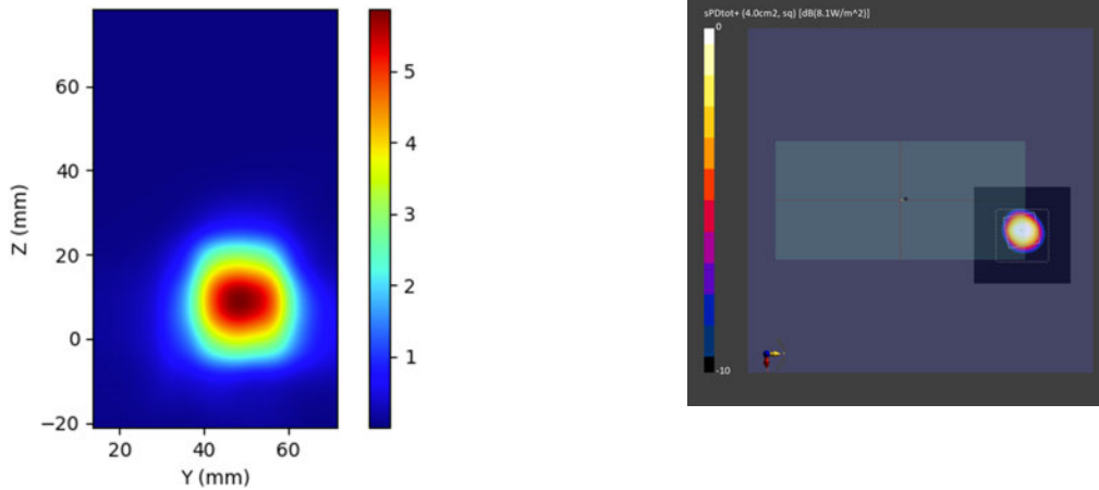
Figure 2-33 Simulated (left) and measured (right) averaged PD distribution for the following configuration: Band n261, MID Channel, Beam ID 4, H polarization, Plane B Module, plotted on the surface S2 (back) with 2mm separation distance to the camera bump.
