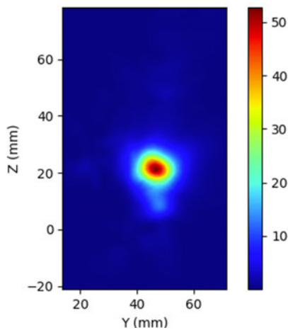
Figure 2-12 Simulated (left) and measured (right) PD distribution for the following configuration: Band n258, MID Channel, Beam ID 1, H+V polarization, Plane B Module, plotted on the surface S2 (back) with 2mm separation distance to the camera bump.
