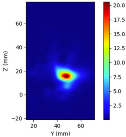
Figure 2-10 Simulated (left) and measured (right) PD distribution for the following configuration: Band n258, MID Channel, Beam ID 2, V polarization, Plane B Module, plotted on the surface S2 (back) with 2mm separation distance to the camera bump.
