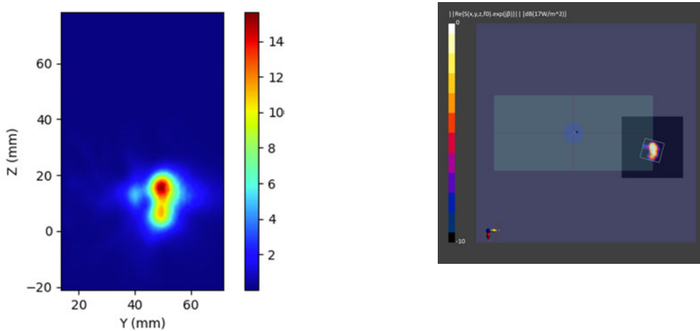
Figure 2-34 Simulated (left) and measured (right) PD distribution for the following configuration: Band n261, MID Channel, Beam ID 3, V polarization, Plane B Module, plotted on the surface S2 (back) with 2mm separation distance to the camera bump.
