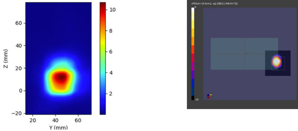
Figure 2-25 Simulated (left) and measured (right) averaged PD distribution for the following configuration: Band n260, MID Channel, Beam ID 3, H+V polarization, Plane B Module, plotted on the surface S2 (back) with 2mm separation distance to the camera bump.
