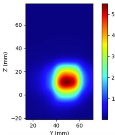
Figure 2-35 Simulated (left) and measured (right) averaged PD distribution for the following configuration: Band n261, MID Channel, Beam ID 3, V polarization, Plane B Module, plotted on the surface S2 (back) with 2mm separation distance to the camera bump.
