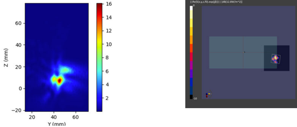
Figure 2-13 Simulated (left) and measured (right) averaged PD distribution for the following configuration: Band n258, MID Channel, Beam ID 1, H+V polarization, Plane B Module, plotted on the surface S2 (back) with 2mm separation distance to the camera bump.
