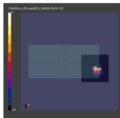
Figure 2-35 Simulated (left) and measured (right) averaged PD distribution for the following configuration: Band n261, MID Channel, Beam ID 3, V polarization, Plane B Module, plotted on the surface S2 (back) with 2mm separation distance to the camera bump.
