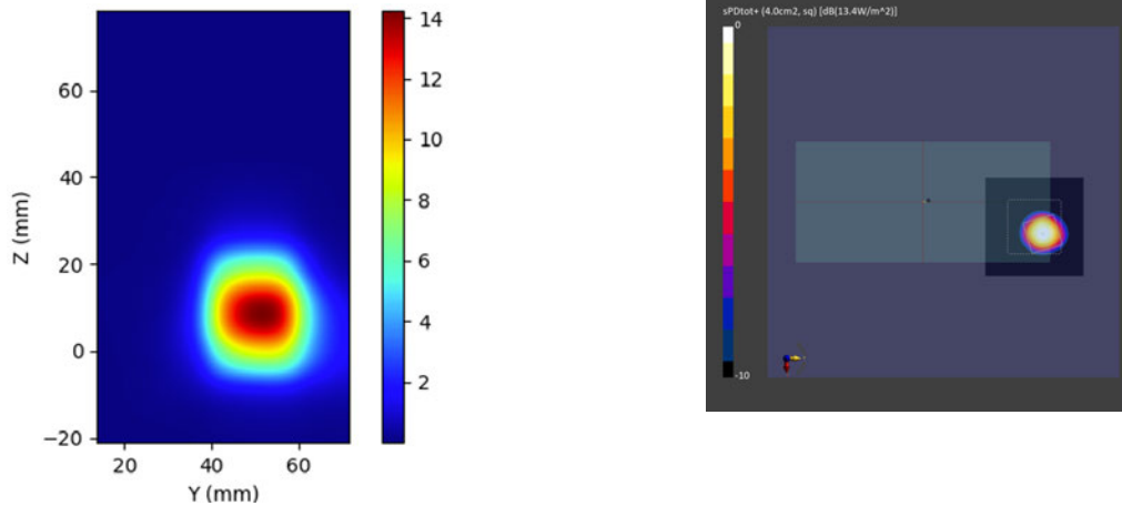
Figure 2-37 Simulated (left) and measured (right) averaged PD distribution for the following configuration: Band n261, MID Channel, Beam ID 4, H+V polarization, Plane B Module, plotted on the surface S2 (back) with 2mm separation distance to the camera bump.
