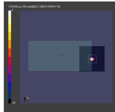
Figure 2-11 Simulated (left) and measured (right) averaged PD distribution for the following configuration: Band n258, MID Channel, Beam ID 2, V polarization, Plane B Module, plotted on the surface S2 (back) with 2mm separation distance to the camera bump.
