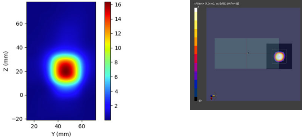
Figure 2-13 Simulated (left) and measured (right) averaged PD distribution for the following configuration: Band n258, MID Channel, Beam ID 1, H+V polarization, Plane B Module, plotted on the surface S2 (back) with 2mm separation distance to the camera bump.
