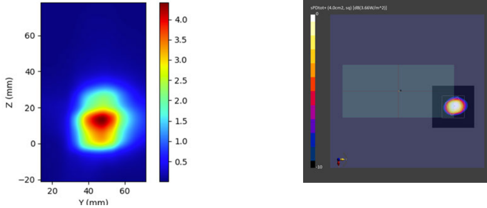
Figure 2-23 Simulated (left) and measured (right) averaged PD distribution for the following configuration: Band n260, MID Channel, Beam ID 3, V polarization, Plane B Module, plotted on the surface S2 (back) with 2mm separation distance to the camera bump.
