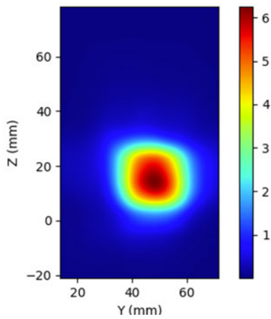
Figure 2-11 Simulated (left) and measured (right) averaged PD distribution for the following configuration: Band n258, MID Channel, Beam ID 2, V polarization, Plane B Module, plotted on the surface S2 (back) with 2mm separation distance to the camera bump.
