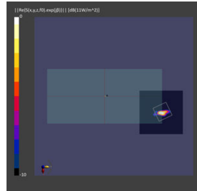
Figure 2-22 Simulated (left) and measured (right) PD distribution for the following configuration: Band n260, MID Channel, Beam ID 3, V polarization, Plane B Module, plotted on the surface S2 (back) with 2mm separation distance to the camera bump.
