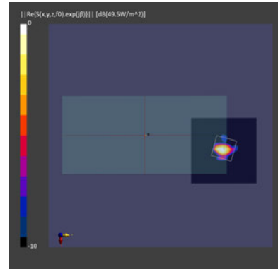
Figure 2-9 Simulated (left) and measured (right) averaged PD distribution for the following configuration: Band n258, MID Channel, Beam ID 4, H polarization, Plane B Module, plotted on the surface S2 (back) with 2mm separation distance to the camera bump.
