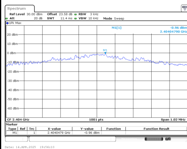
Power Density (dBm/3kHz) Plot Channel 02
