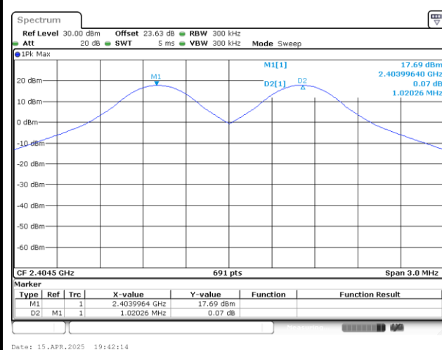
Channel Separation Plot on Channel 02 - 03
