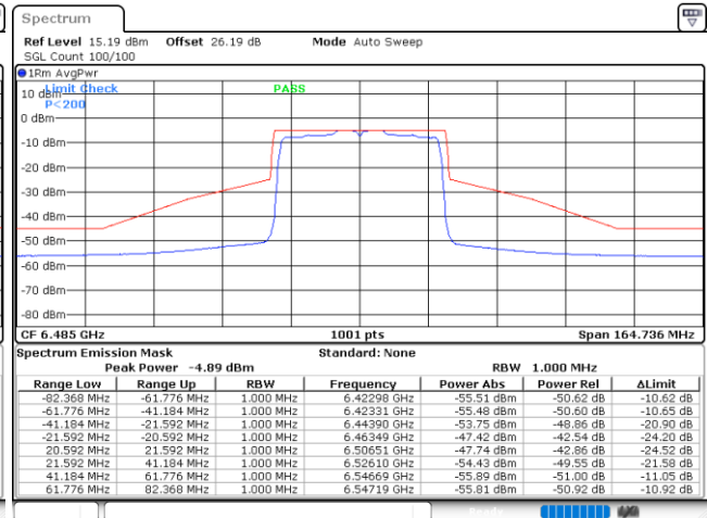
Plot on 6485 MHz
