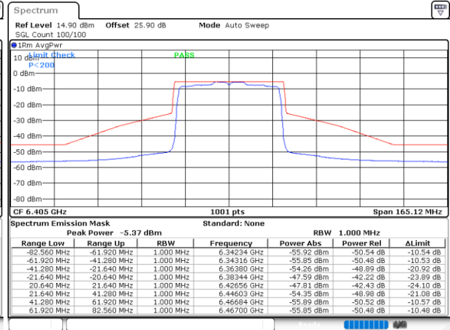
Plot on 6405 MHz
