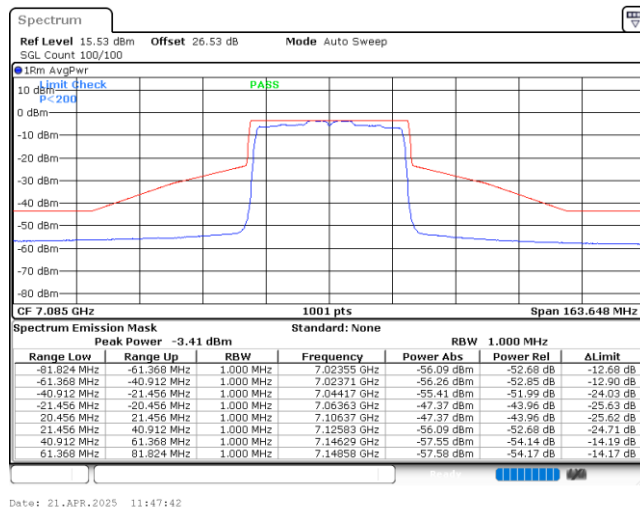
Plot on 7085 MHz
