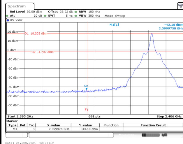
Low Band Edge Plot on Channel 02
