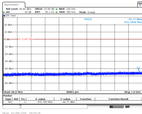
CSE Plot on High Ch between 30MHz ~ 1 GHz
