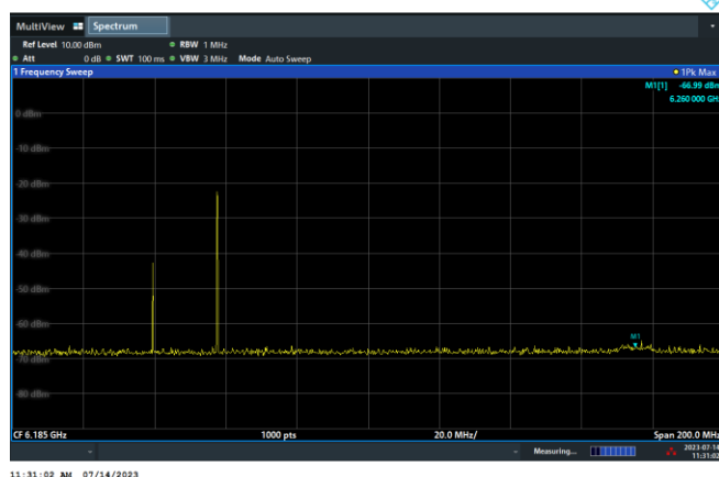
After 10MHz incumbent injected on top of channel, the entire 160MHz bandwidth stops transmission.
