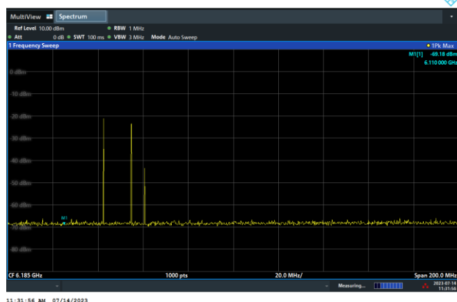
After 10MHz incumbent injected on bottom of channel, the entire 160MHz bandwidth stops transmission.
