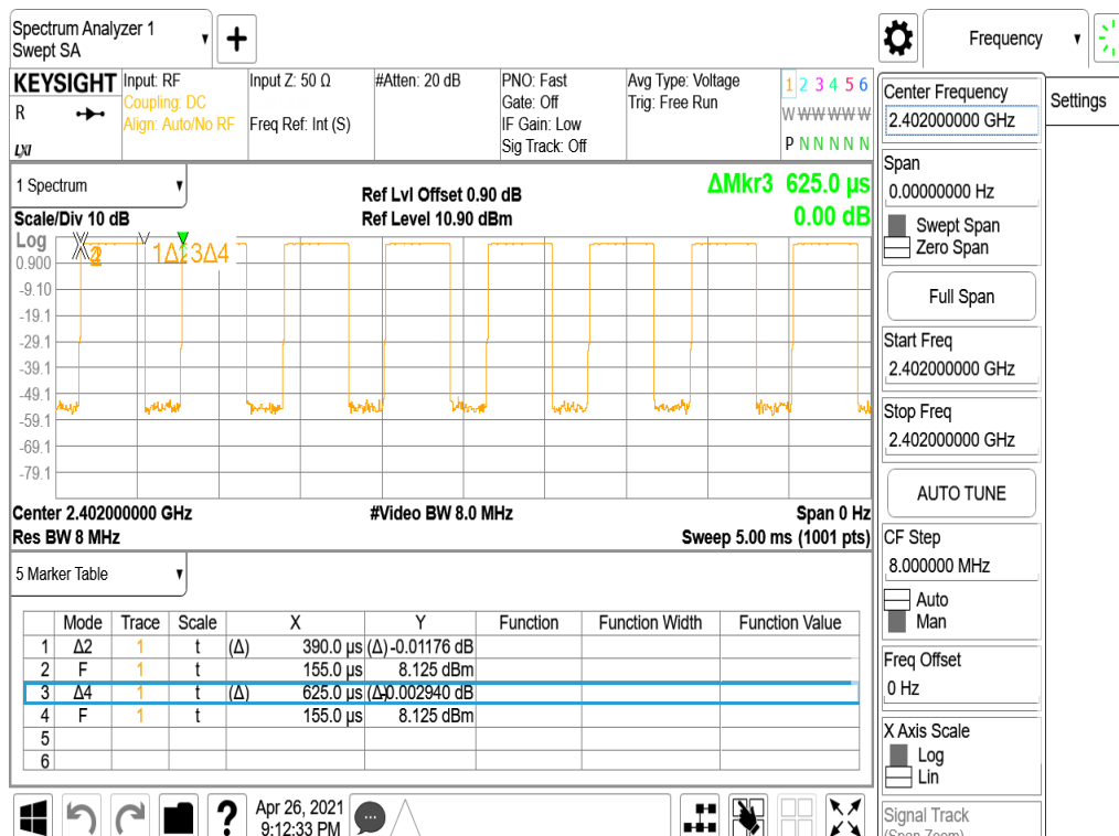
BLE_1M_LowCH00-2402
