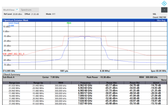
Plot on Channel 6995 MHz
