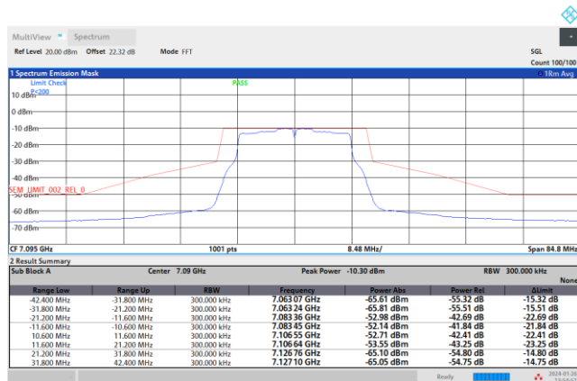
Plot on Channel 7095 MHz
