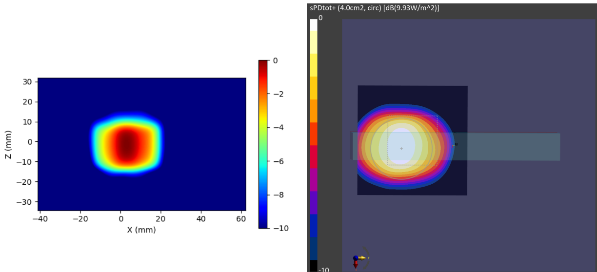
Figure 2-19 Simulated (left) and measured (right) averaged PD distribution for the following configuration: Band n261, MID Channel, Beam ID 3, H+V polarization, Plane A Module, plotted on the surface S5 (top) with 2mm separation distance to the DUT.
