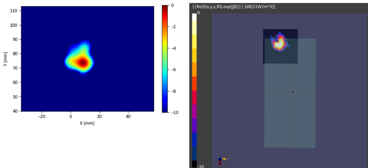
Figure 2-34 Simulated (left) and measured (right) PD distribution for the following configuration: Band n258, MID Channel, Beam ID 4, V polarization, Plane B Module, plotted on the surface S2 (back) with 2mm separation distance to the camera bump.
