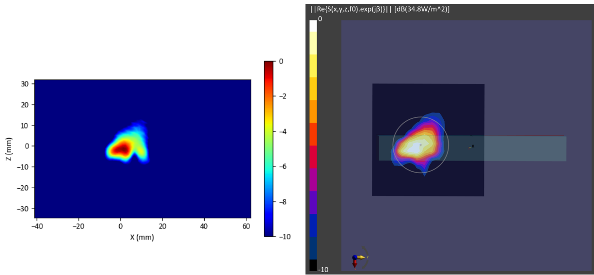
Figure 2-26 Simulated (left) and measured (right) PD distribution for the following configuration: Band n258, MID Channel, Beam ID 4, H polarization, Plane A Module, plotted on the surface S5 (top) with 2mm separation distance to the DUT.
