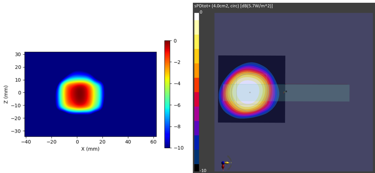
Figure 2-15 Simulated (left) and measured (right) averaged PD distribution for the following configuration: Band n261, MID Channel, Beam ID 3, H polarization, Plane A Module, plotted on the surface S5 (top) with 2mm separation distance to the DUT.
