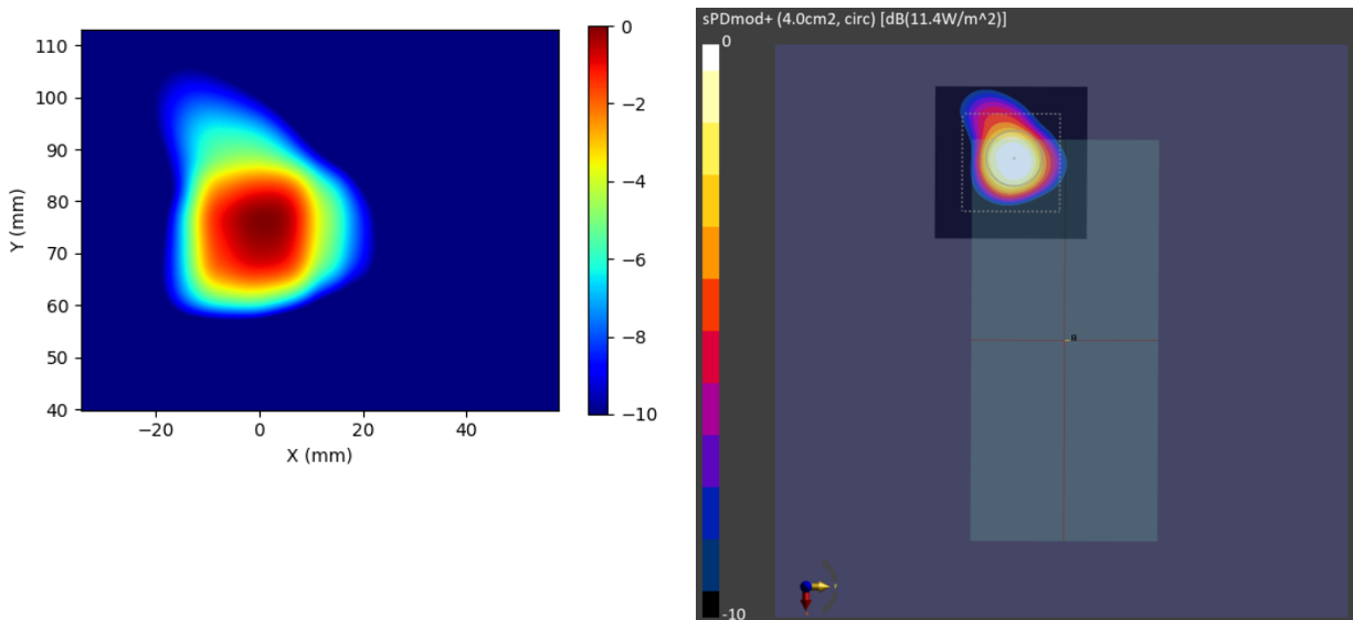
Figure 2-25 Simulated (left) and measured (right) averaged PD distribution for the following configuration: Band n261, MID Channel, Beam ID 1, H+V polarization, Plane B Module, plotted on the surface S2 (back) with 2mm separation distance to the camera bump.
