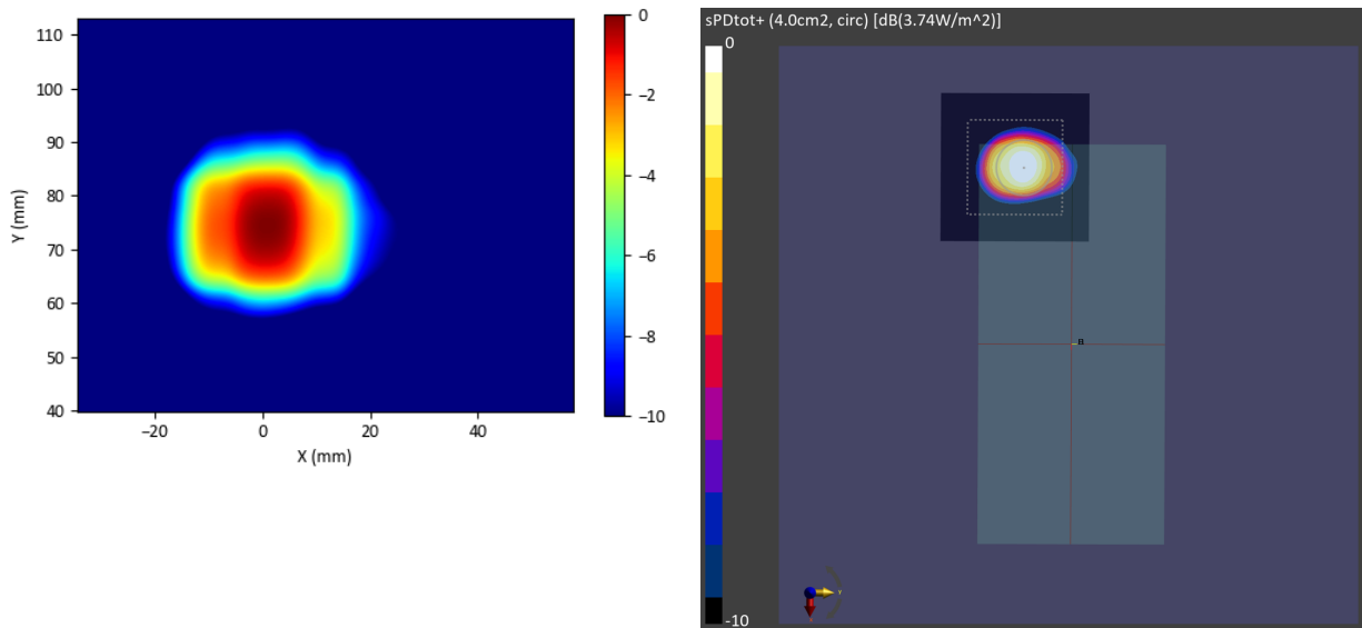
Figure 2-11 Simulated (left) and measured (right) averaged PD distribution for the following configuration: Band n260, MID Channel, Beam ID 2, V polarization, Plane B Module, plotted on the surface S2 (back) with 2mm separation distance to the camera bump.
