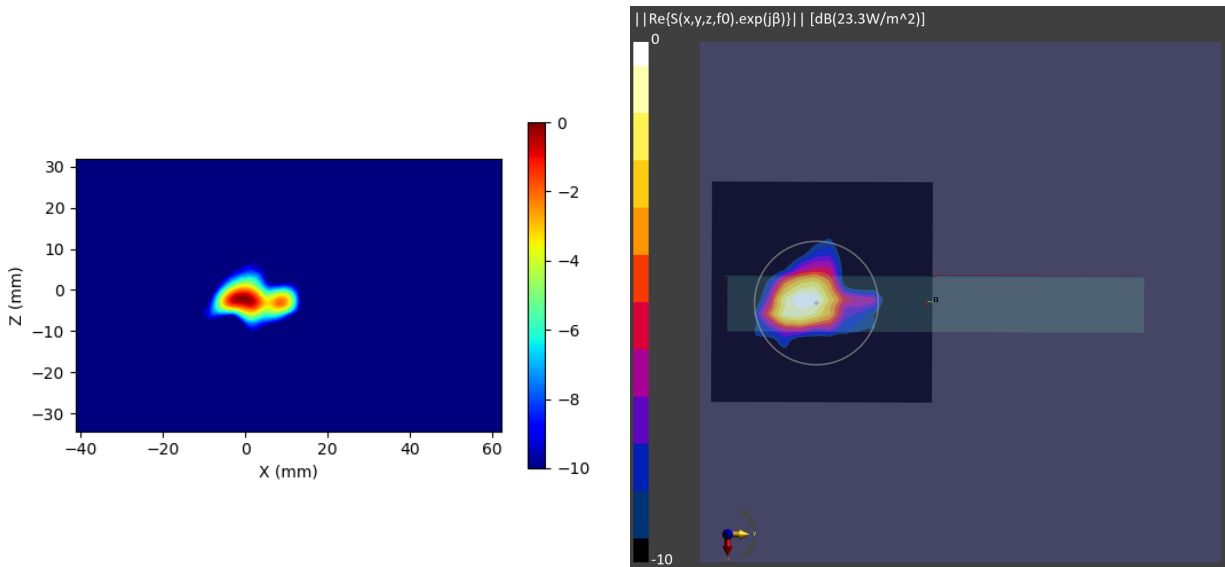
Figure 2-14 Simulated (left) and measured (right) PD distribution for the following configuration: Band n261, MID Channel, Beam ID 3, H polarization, Plane A Module, plotted on the surface S5 (top) with 2mm separation distance to the DUT.
