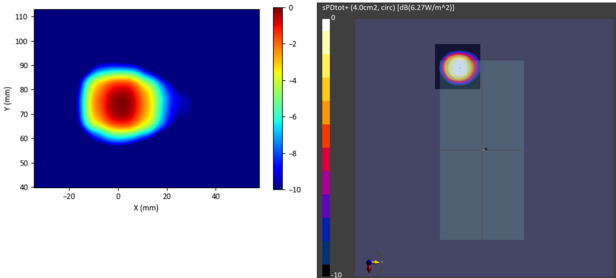
Figure 2-13 Simulated (left) and measured (right) averaged PD distribution for the following configuration: Band n260, MID Channel, Beam ID 2, H+V polarization, Plane B Module, plotted on the surface S2 (back) with 2mm separation distance to the camera bump.
