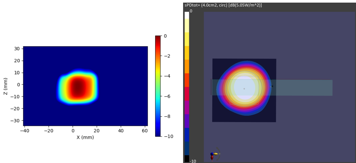
Figure 2-17 Simulated (left) and measured (right) averaged PD distribution for the following configuration: Band n261, MID Channel, Beam ID 4, V polarization, Plane A Module, plotted on the surface S5 (top) with 2mm separation distance to the DUT.
