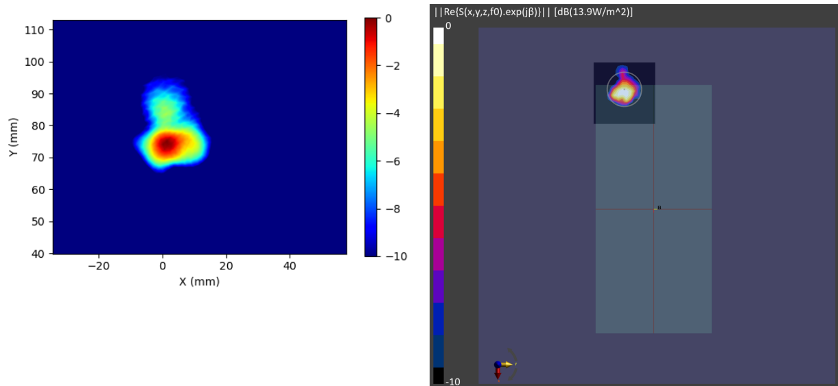
Figure 2-20 Simulated (left) and measured (right) PD distribution for the following configuration: Band n261, MID Channel, Beam ID 2, H polarization, Plane B Module, plotted on the surface S2 (back) with 2mm separation distance to the camera bump.
