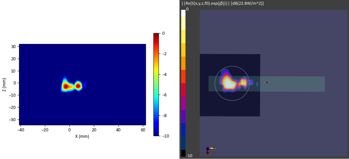
Figure 2-2 Simulated (left) and measured (right) PD distribution for the following configuration: Band n260, MID Channel, Beam ID 1, H polarization, Plane A Module, plotted on the surface S5 (top) with 2mm separation distance to the DUT.
