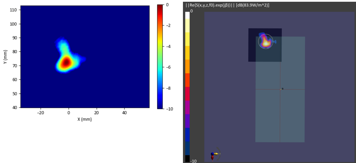
Figure 2-36 Simulated (left) and measured (right) PD distribution for the following configuration: Band n258, MID Channel, Beam ID 1, H+V polarization, Plane B Module, plotted on the surface S2 (back) with 2mm separation distance to the camera bump.
