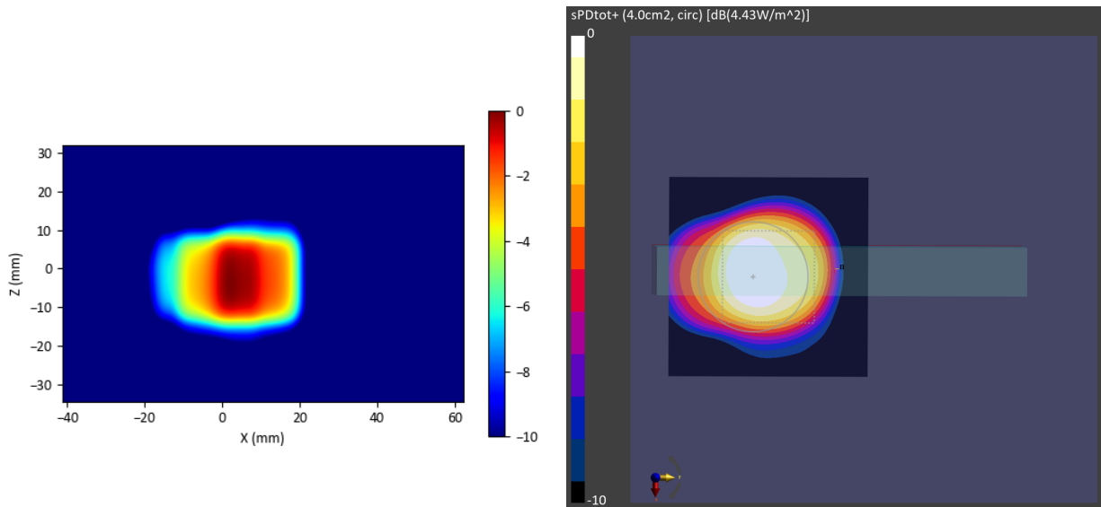
Figure 2-5 Simulated (left) and measured (right) averaged PD distribution for the following configuration: Band n260, MID Channel, Beam ID 5, V polarization, Plane A Module, plotted on the surface S5 (top) with 2mm separation distance to the DUT.
