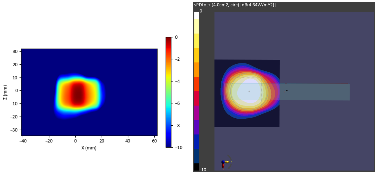
Figure 2-3 Simulated (left) and measured (right) averaged PD distribution for the following configuration: Band n260, MID Channel, Beam ID 1, H polarization, Plane A Module, plotted on the surface S5 (top) with 2mm separation distance to the DUT.
