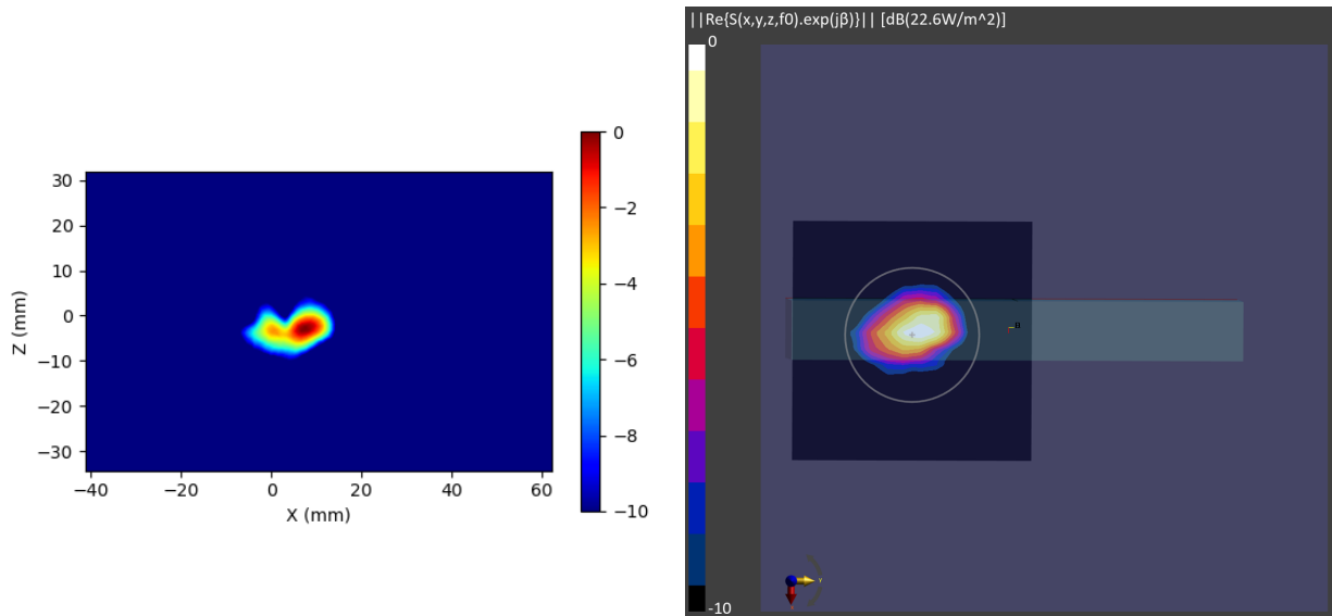
Figure 2-16 Simulated (left) and measured (right) PD distribution for the following configuration: Band n261, MID Channel, Beam ID 4, V polarization, Plane A Module, plotted on the surface S5 (top) with 2mm separation distance to the DUT.
