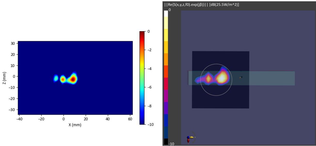
Figure 2-4 Simulated (left) and measured (right) PD distribution for the following configuration: Band n260, MID Channel, Beam ID 5, V polarization, Plane A Module, plotted on the surface S5 (top) with 2mm separation distance to the DUT.
