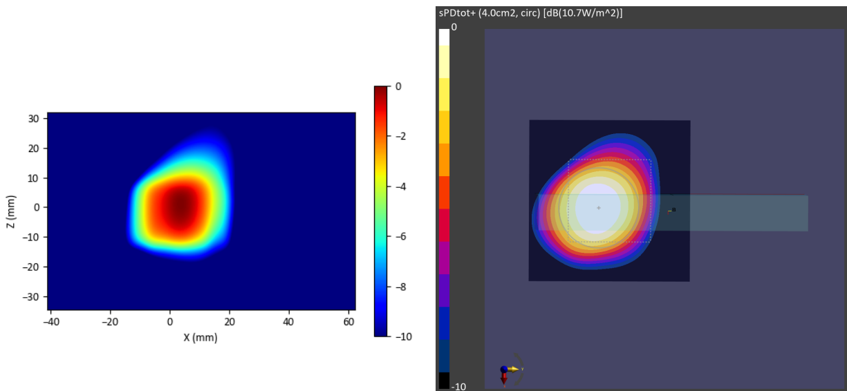
Figure 2-27 Simulated (left) and measured (right) averaged PD distribution for the following configuration: Band n258, MID Channel, Beam ID 4, H polarization, Plane A Module, plotted on the surface S5 (top) with 2mm separation distance to the DUT.
