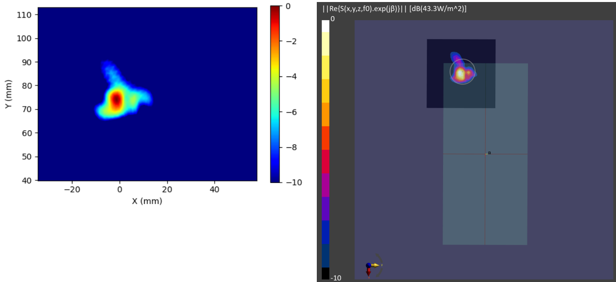
Figure 2-24 Simulated (left) and measured (right) PD distribution for the following configuration: Band n261, MID Channel, Beam ID 1, H+V polarization, Plane B Module, plotted on the surface S2 (back) with 2mm separation distance to the camera bump.
