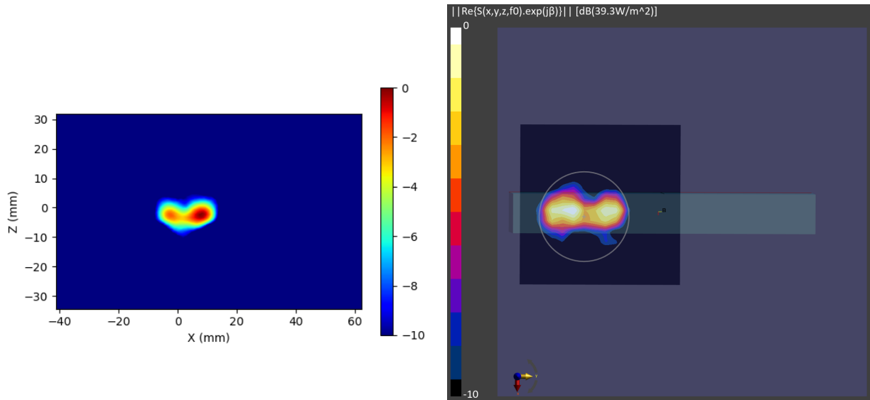
Figure 2-18 Simulated (left) and measured (right) PD distribution for the following configuration: Band n261, MID Channel, Beam ID 3, H+V polarization, Plane A Module, plotted on the surface S5 (top) with 2mm separation distance to the DUT.
