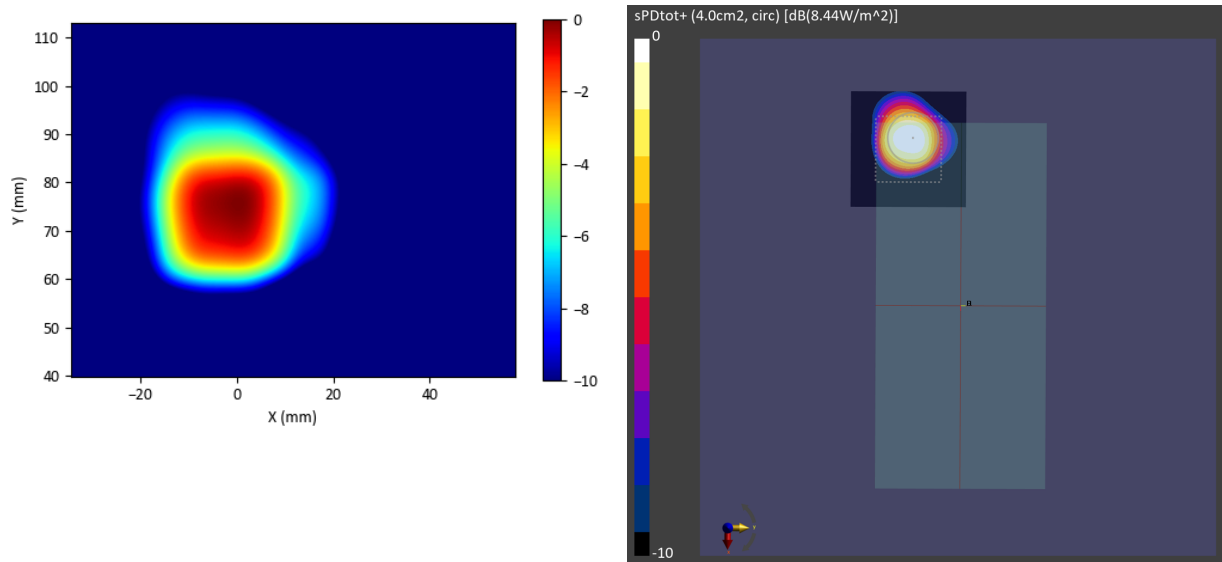
Figure 2-33 Simulated (left) and measured (right) averaged PD distribution for the following configuration: Band n258, MID Channel, Beam ID 1, H polarization, Plane B Module, plotted on the surface S2 (back) with 2mm separation distance to the camera bump.
