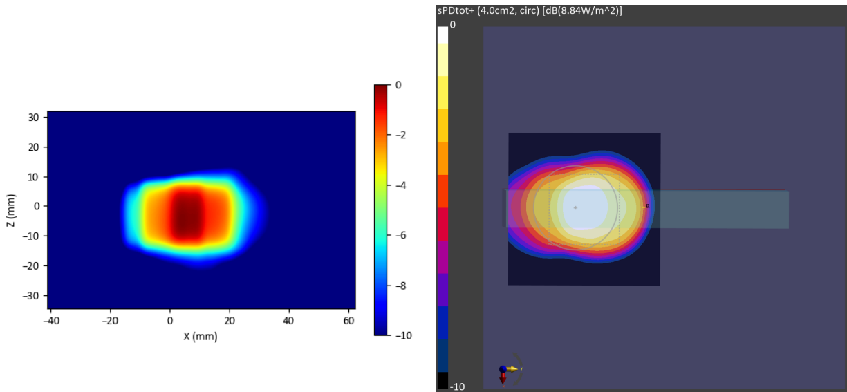
Figure 2-7 Simulated (left) and measured (right) averaged PD distribution for the following configuration: Band n260, MID Channel, Beam ID 6, H+V polarization, Plane A Module, plotted on the surface S5 (top) with 2mm separation distance to the DUT.
