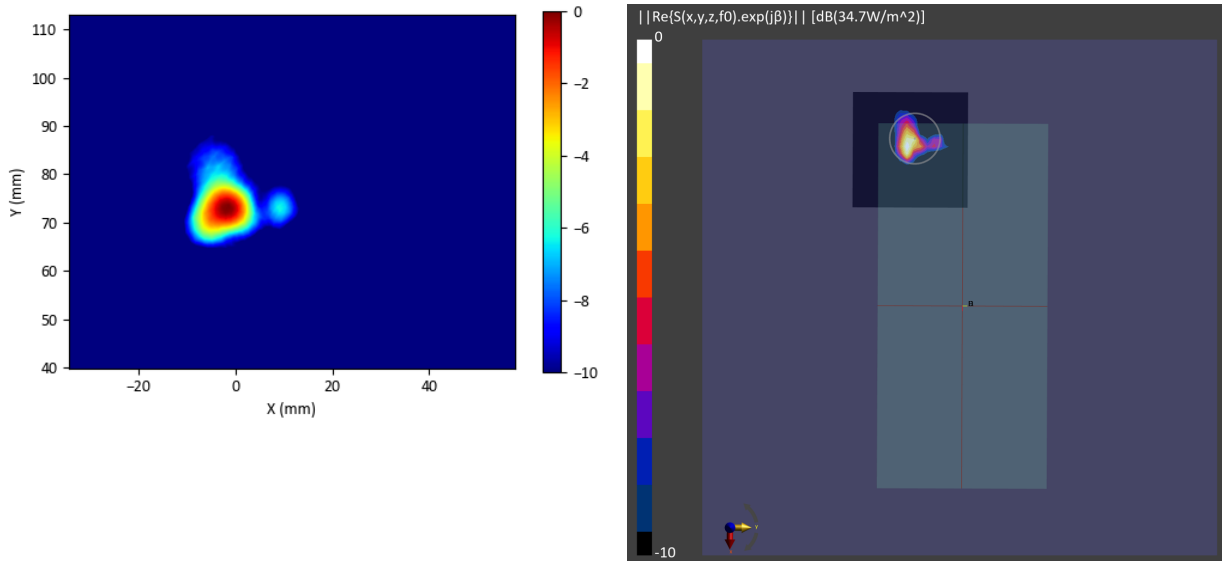
Figure 2-32 Simulated (left) and measured (right) PD distribution for the following configuration: Band n258, MID Channel, Beam ID 1, H polarization, Plane B Module, plotted on the surface S2 (back) with 2mm separation distance to the camera bump.
