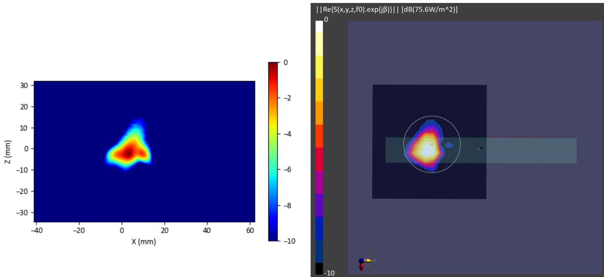
Figure 2-30 Simulated (left) and measured (right) PD distribution for the following configuration: Band n258, MID Channel, Beam ID 4, H+V polarization, Plane A Module, plotted on the surface S5 (top) with 2mm separation distance to the DUT.
