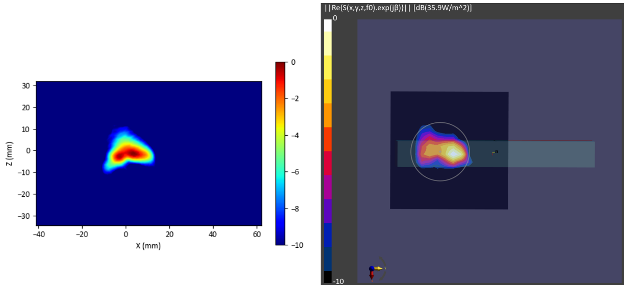
Figure 2-28 Simulated (left) and measured (right) PD distribution for the following configuration: Band n258, MID Channel, Beam ID 2, V polarization, Plane A Module, plotted on the surface S5 (top) with 2mm separation distance to the DUT.
