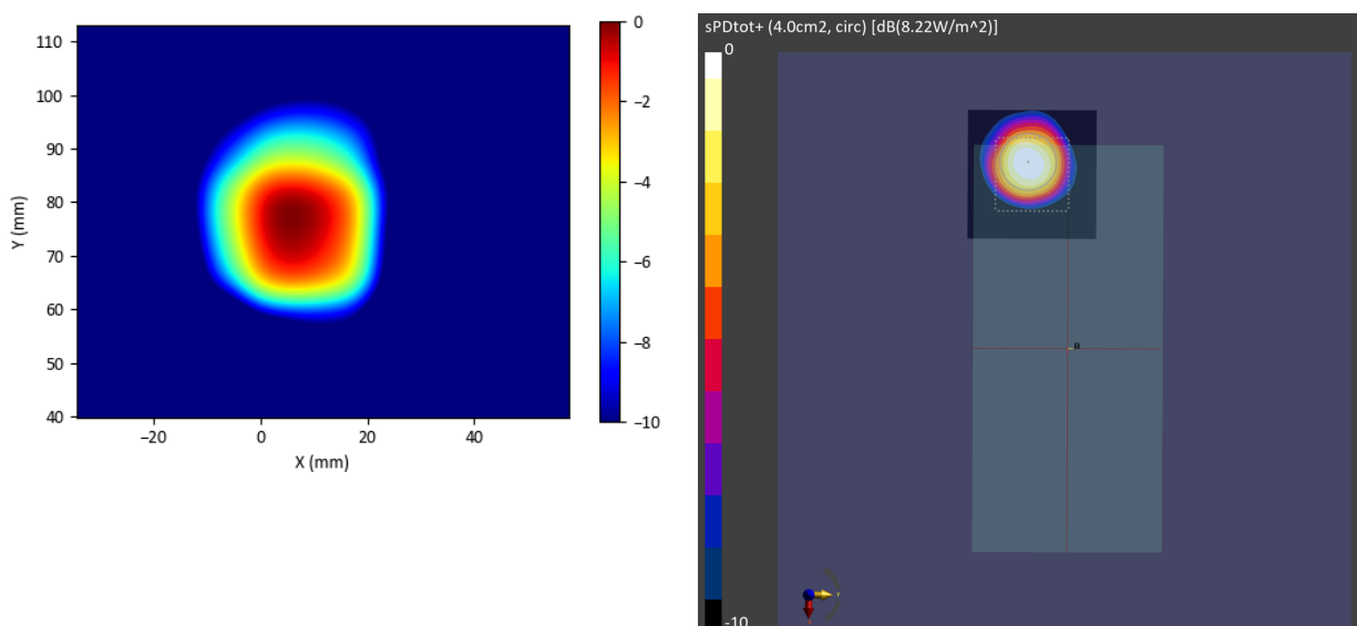
Figure 2-35 Simulated (left) and measured (right) averaged PD distribution for the following configuration: Band n258, MID Channel, Beam ID 4, V polarization, Plane B Module, plotted on the surface S2 (back) with 2mm separation distance to the camera bump.
