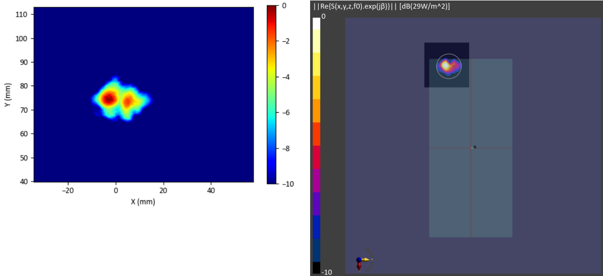
Figure 2-12 Simulated (left) and measured (right) PD distribution for the following configuration: Band n260, MID Channel, Beam ID 2, H+V polarization, Plane B Module, plotted on the surface S2 (back) with 2mm separation distance to the camera bump.
