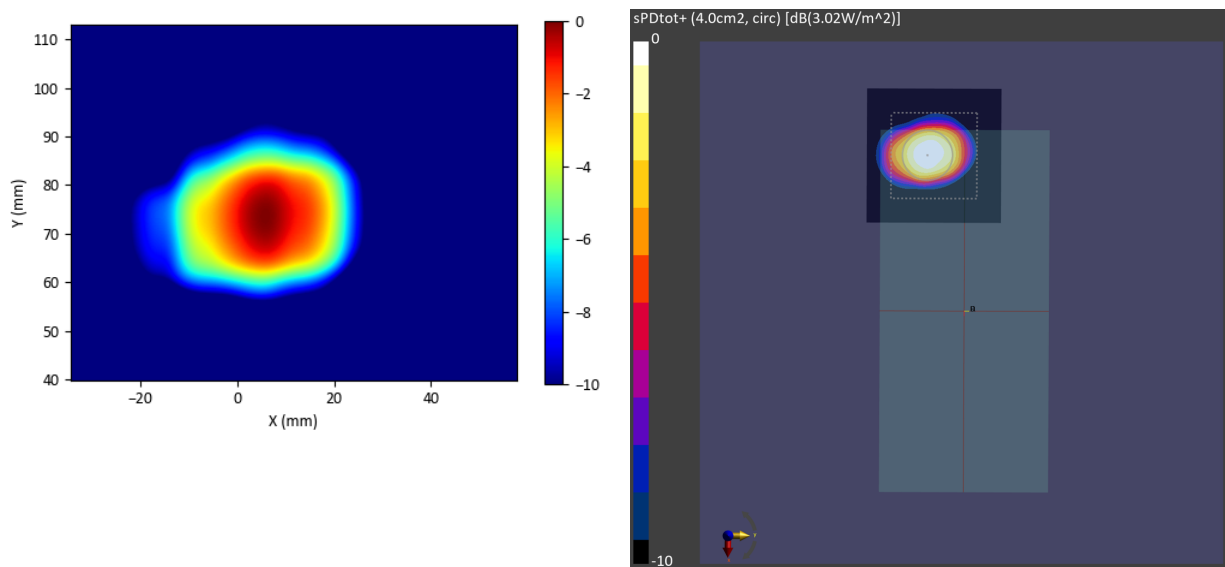
Figure 2-9 Simulated (left) and measured (right) averaged PD distribution for the following configuration: Band n260, MID Channel, Beam ID 4, H polarization, Plane B Module, plotted on the surface S2 (back) with 2mm separation distance to the camera bump.
