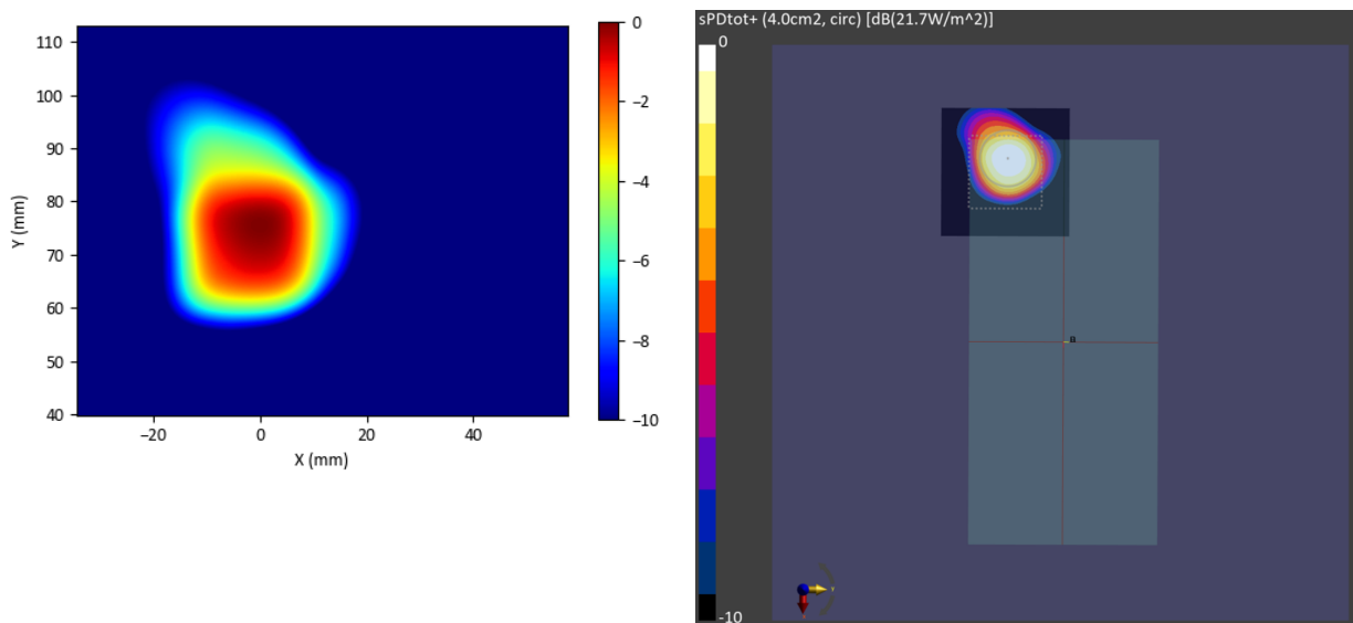
Figure 2-37 Simulated (left) and measured (right) averaged PD distribution for the following configuration: Band n258, MID Channel, Beam ID 1, H+V polarization, Plane B Module, plotted on the surface S2 (back) with 2mm separation distance to the camera bump.
