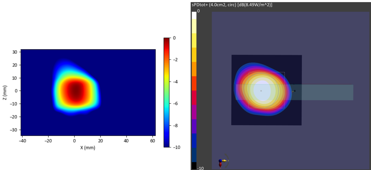
Figure 2-29 Simulated (left) and measured (right) averaged PD distribution for the following configuration: Band n258, MID Channel, Beam ID 2, V polarization, Plane A Module, plotted on the surface S5 (top) with 2mm separation distance to the DUT.
