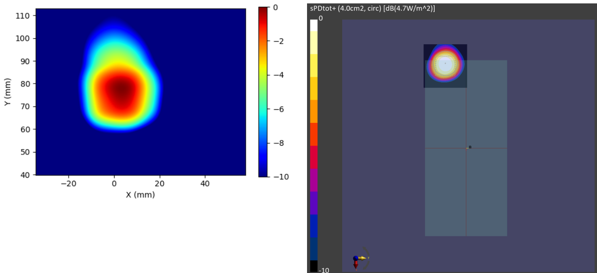
Figure 2-21 Simulated (left) and measured (right) averaged PD distribution for the following configuration: Band n261, MID Channel, Beam ID 2, H polarization, Plane B Module, plotted on the surface S2 (back) with 2mm separation distance to the camera bump.
