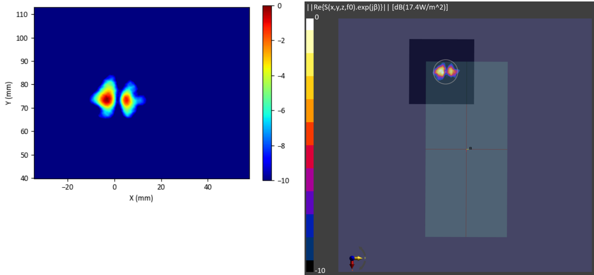
Figure 2-10 Simulated (left) and measured (right) PD distribution for the following configuration: Band n260, MID Channel, Beam ID 2, V polarization, Plane B Module, plotted on the surface S2 (back) with 2mm separation distance to the camera bump.
