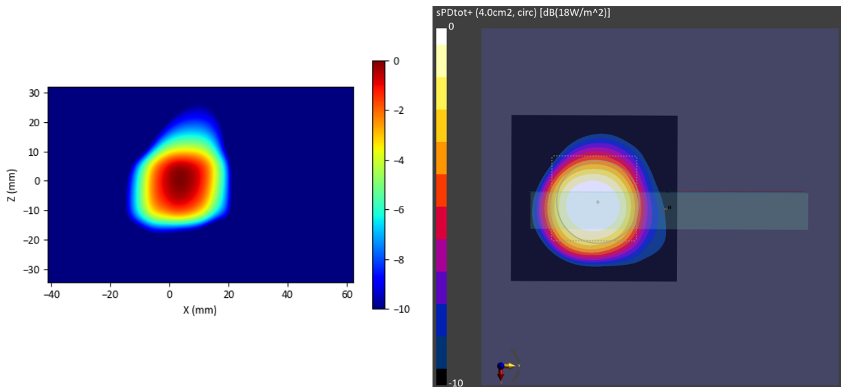
Figure 2-31 Simulated (left) and measured (right) averaged PD distribution for the following configuration: Band n258, MID Channel, Beam ID 4, H+V polarization, Plane A Module, plotted on the surface S5 (top) with 2mm separation distance to the DUT.
