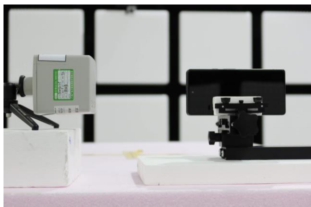
Position E, test separation 15 cm
