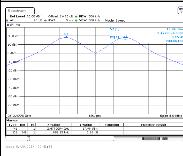
Channel Separation Plot on Channel 75 - 76
