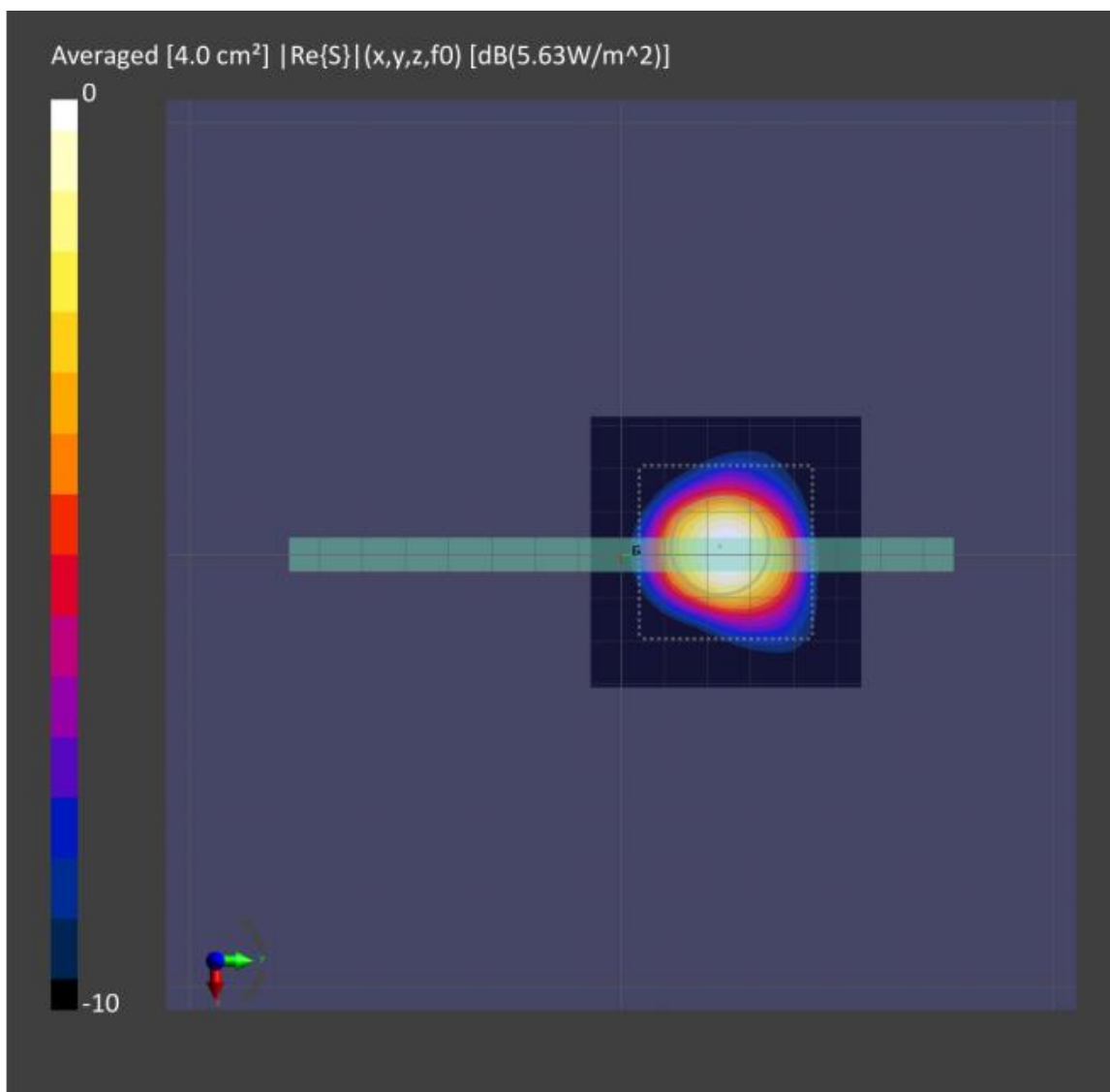
Figure 7-2: 4cm2-averaged power density distribution measured at input.power.limit of 4.118 dBm on the Right Side surface for n261 beam 22
