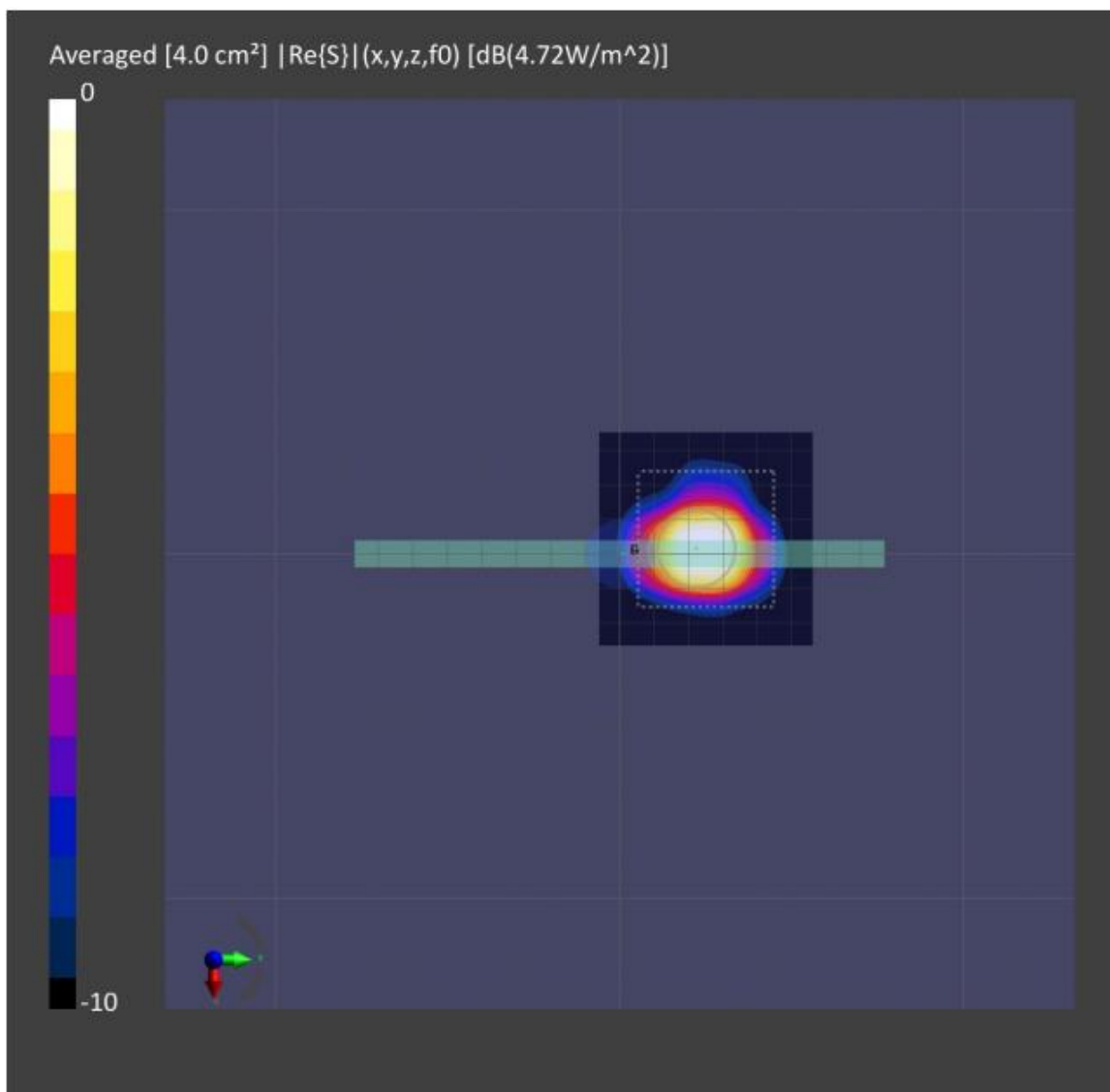
Figure 7-3: 4cm2-averaged power density distribution measured at input.power.limit of 3.9 dBm on the Right Side for n260 beam 16
