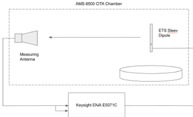
Figure: Block Diagram of Path Loss
