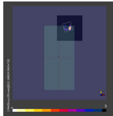
Figure 2-24 Simulated (left) and measured (right) PD distribution for the following configuration: Band n260, MID Channel, Beam ID 3, H+V polarization, Plane B Module, plotted on the surface S2 (back) with 2mm separation distance to the camera bump.
