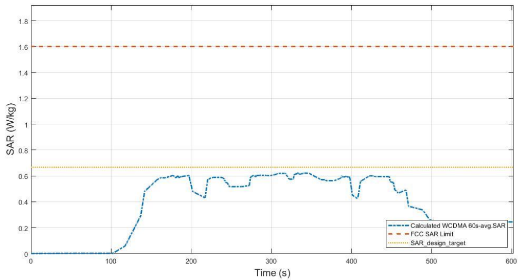
Figure 7.3-14 Total time-averaged SAR
