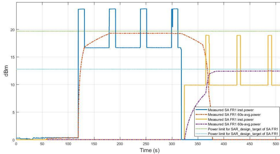
Figure 7.4-1 Conducted Tx power for SAR states change
