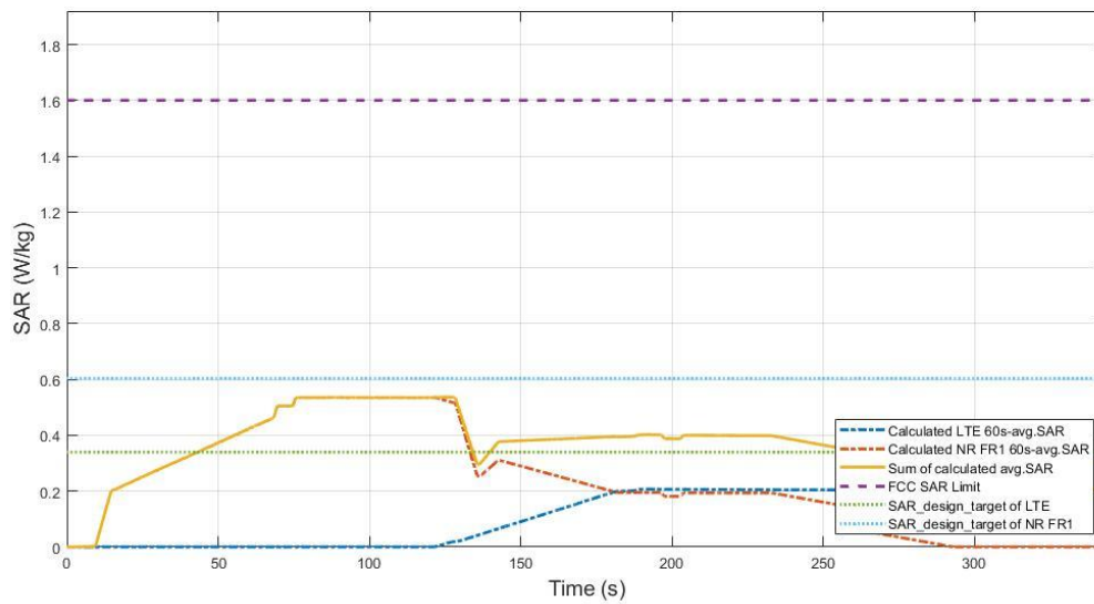
Figure 7.7-2 Total time-averaged SAR
