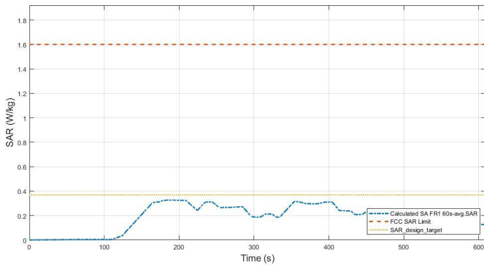
Figure 7.3-22 Total time-averaged SAR
