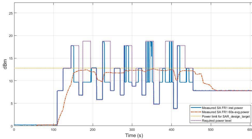
Figure 7.3-23 Conducted Tx power
