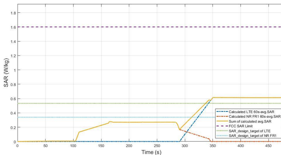
Figure 7.8-2 Total time-averaged SAR
