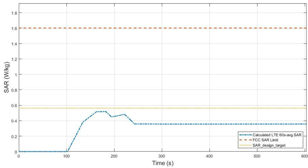
Figure 7.3-8 Total time-averaged SAR
