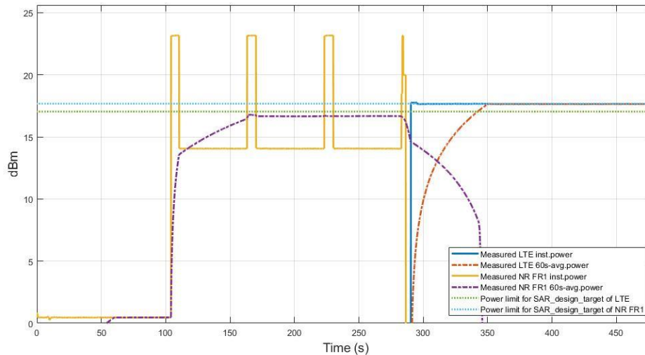
Figure 7.8-1 Conducted Tx power for SAR IRAT re-selection
