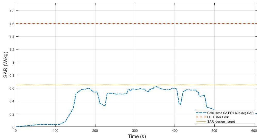
Figure 7.3-24 Total time-averaged SAR
