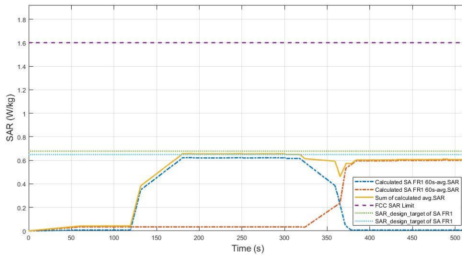
Figure 7.4-2 Total time-averaged SAR
