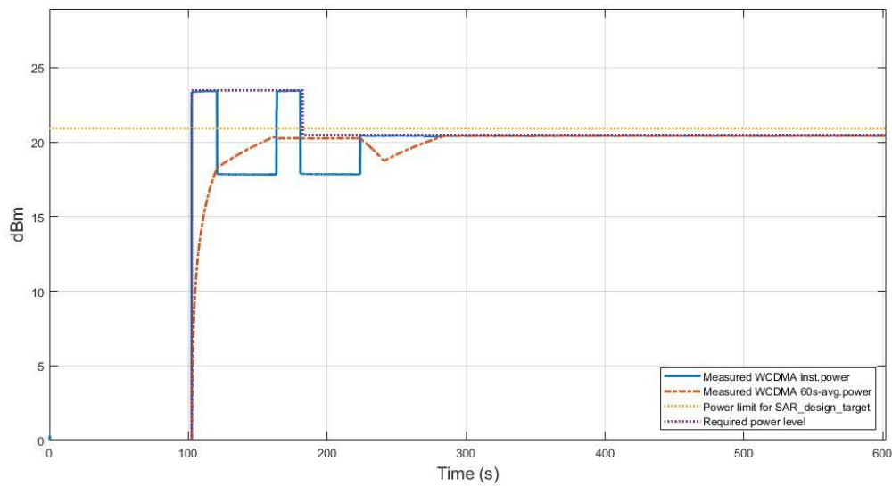
Figure 7.3-3 Time-average conducted power
