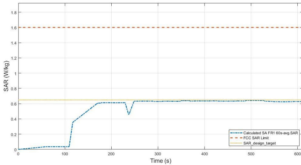
Figure 7.3-12 Total time-averaged SAR in F_TC04
