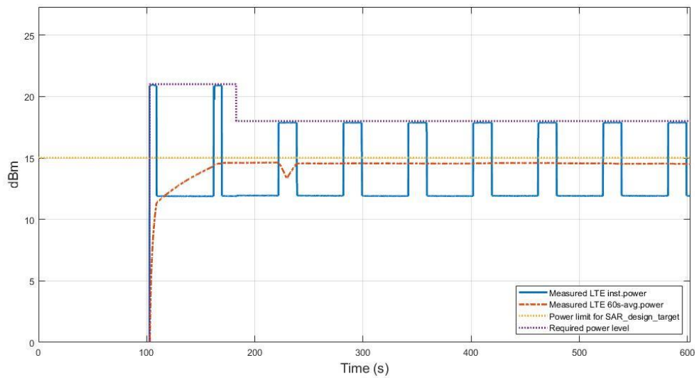
Figure 7.3-5 Time-average conducted power
