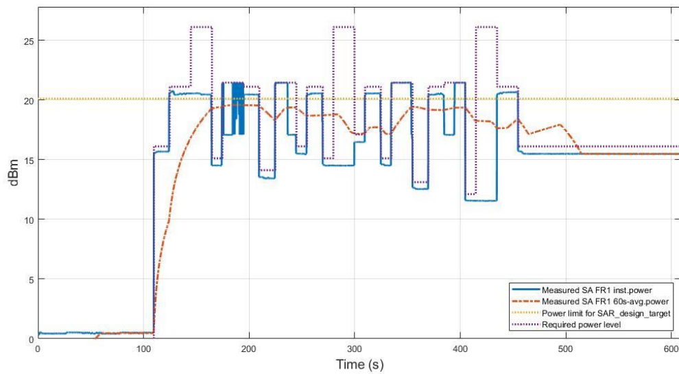
Figure 7.3-21 Conducted Tx power
