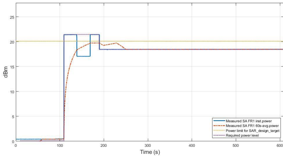
Figure 7.3-9 Conducted Tx power
