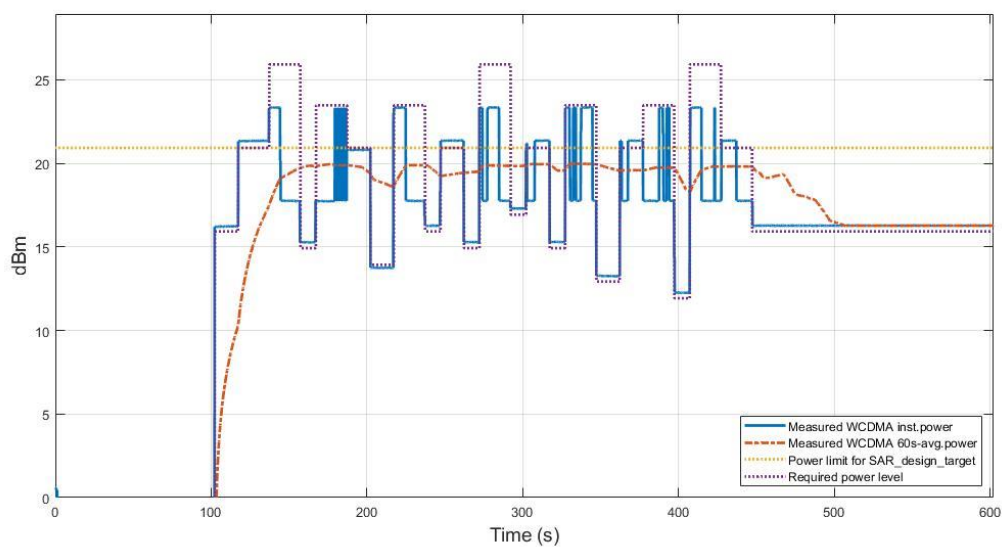
Figure 7.3-15 Conducted Tx power
