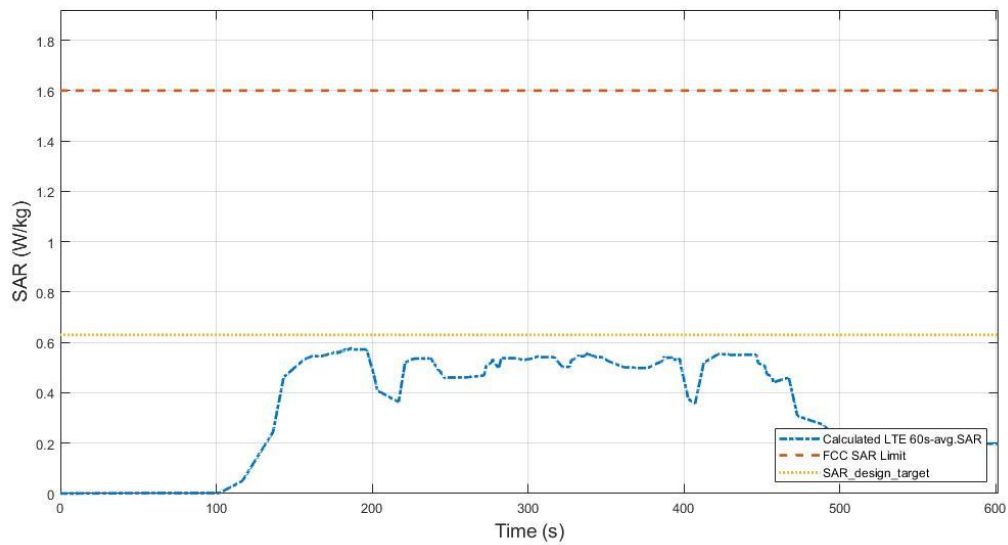
Figure 7.3-18 Total time-averaged SAR
