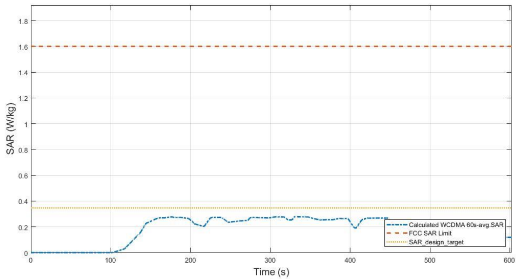
Figure 7.3-16 Total time-averaged SAR
