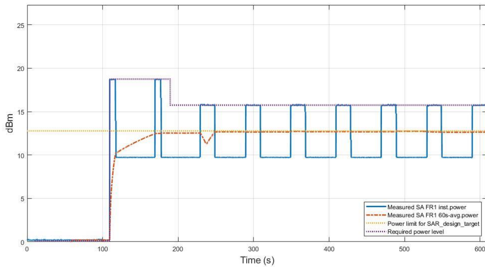
Figure 7.3-11 Conducted Tx power
