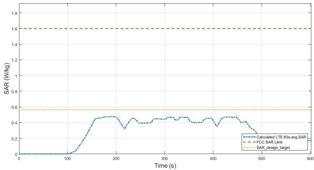
Figure 7.3-20 Total time-averaged SAR
