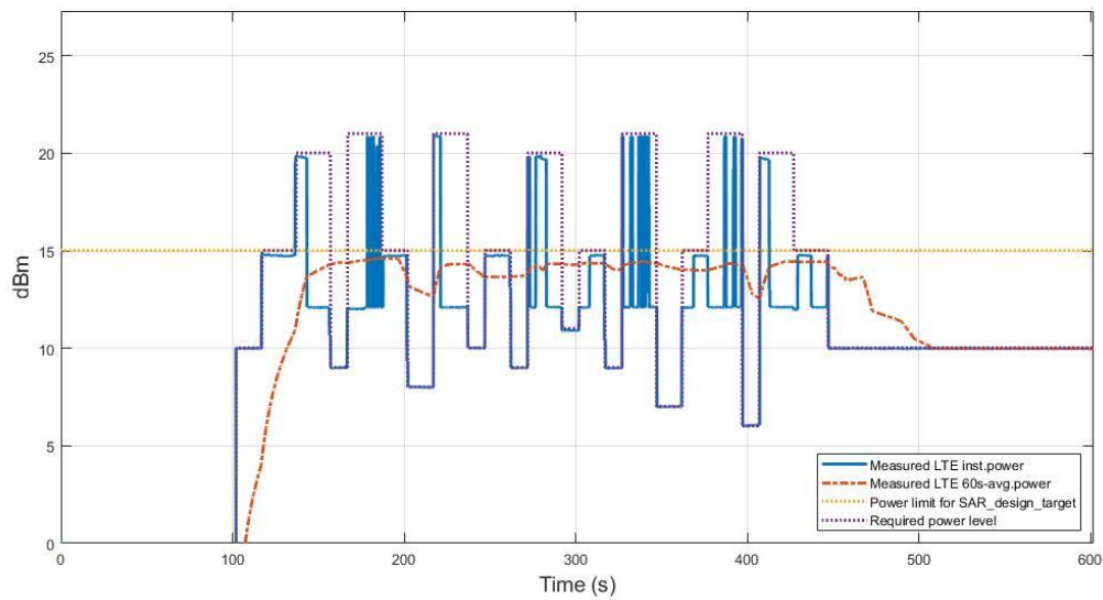
Figure 7.3-17 Conducted Tx power
