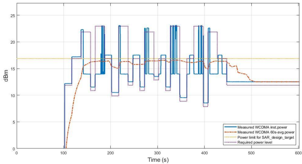
Figure 7.3-13 Conducted Tx power
