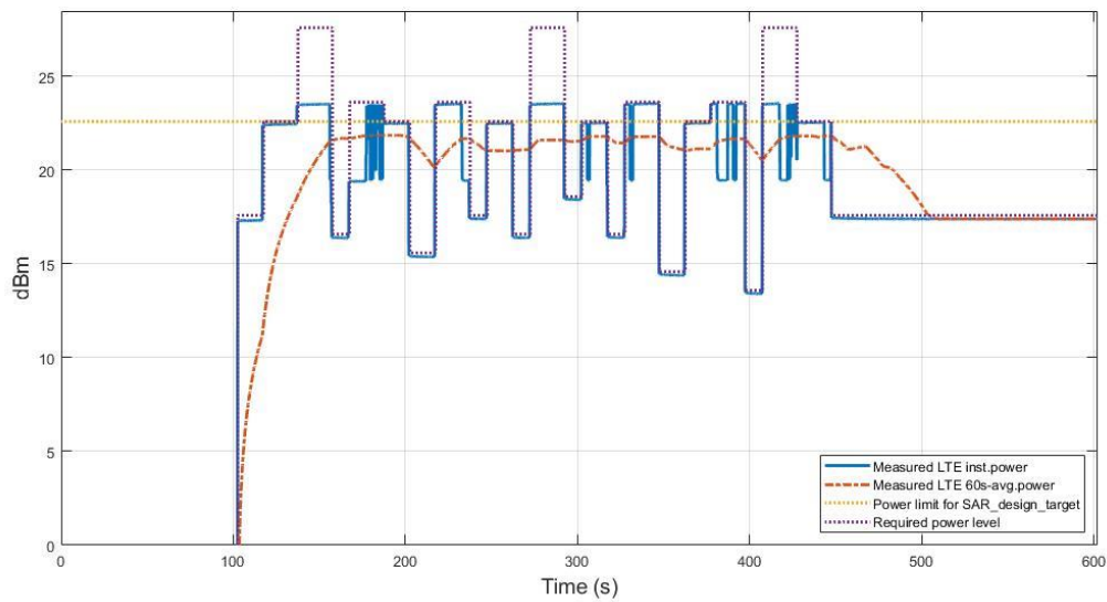
Figure 7.3-19 Conducted Tx power
