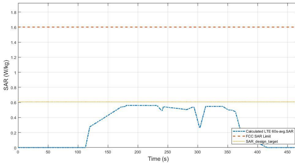
Figure 7.9-2 Total time-averaged SAR
