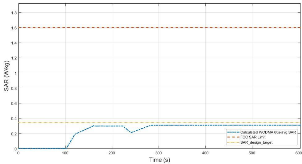
Figure 7.3-4 Total time-averaged SAR
