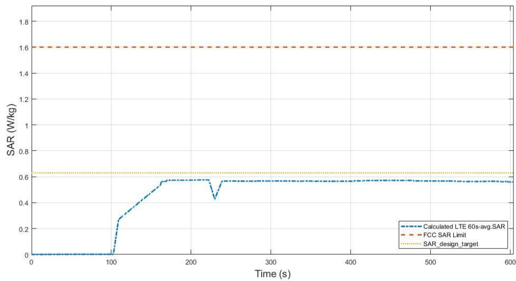
Figure 7.3-6 Total time-averaged SAR
