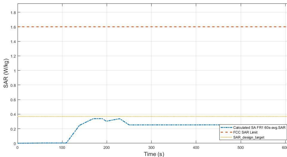
Figure 7.3-10 Total time-averaged SAR
