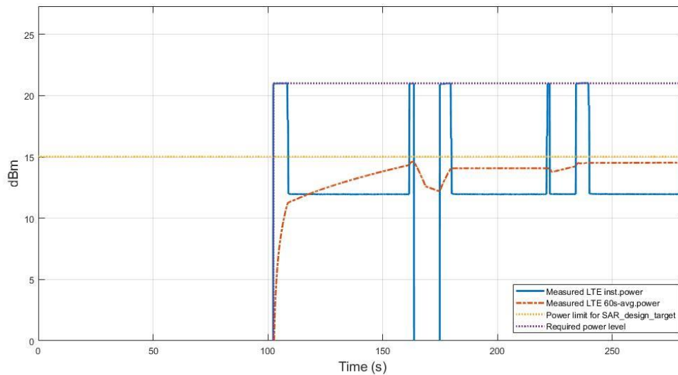
Figure 7.6-1 Conducted Tx power in Call_Disconnect_Reestablishment
