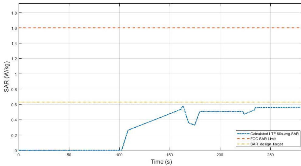
Figure 7.6-2 Total time-averaged SAR
