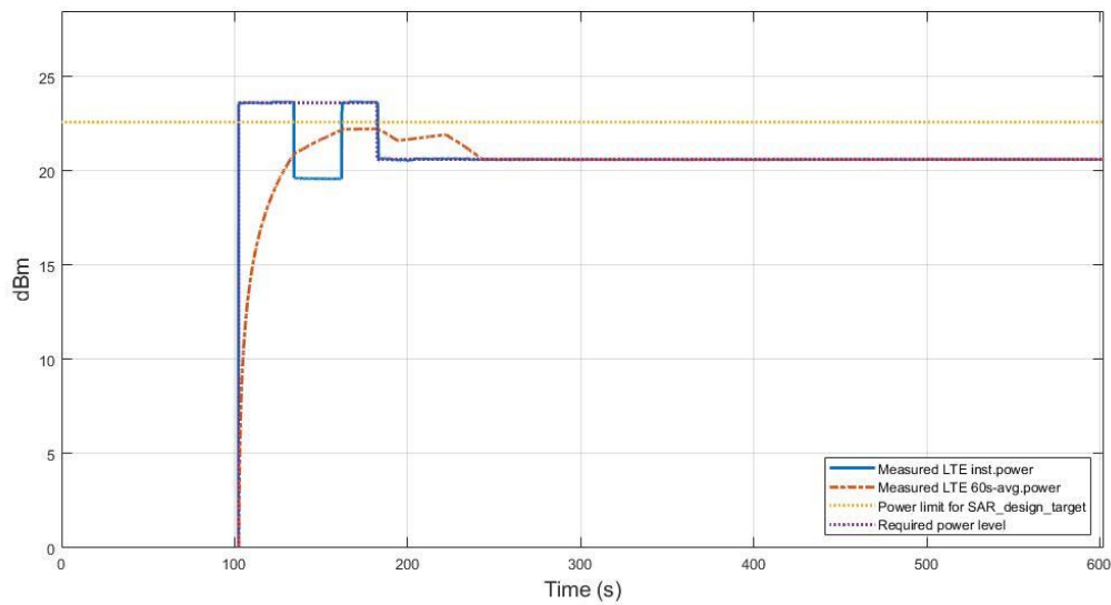
Figure 7.3-7 Time-average conducted power
