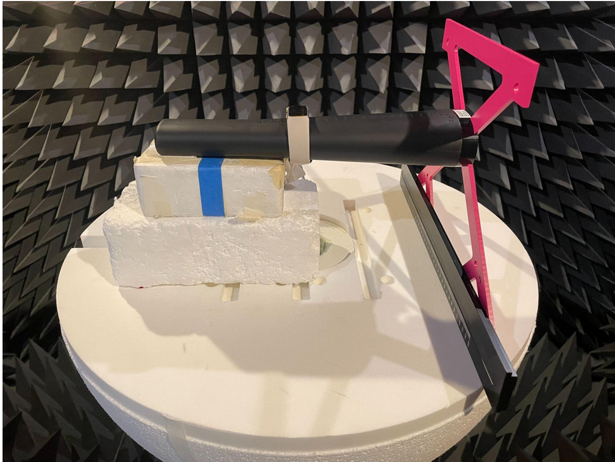
Antenna Test Setup Photo
