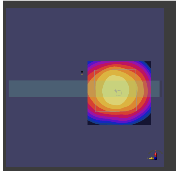
Figure 2-27 Simulated (left) and measured (right) averaged PD distribution for the following configuration: Band n258, MID Channel, Beam ID 0, H polarization, Plane A Module, plotted on the surface S5 (top) with 2mm separation distance to the DUT.
