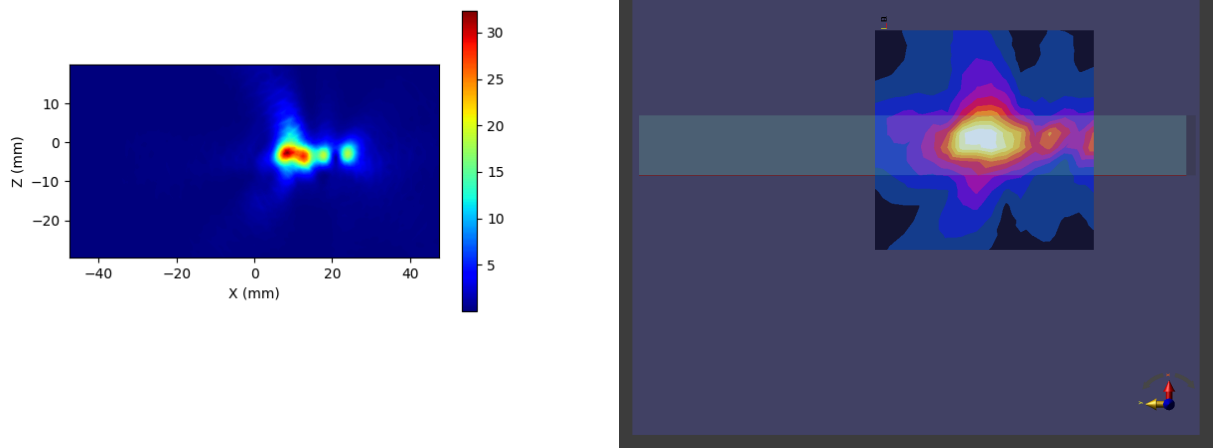
Figure 2-2 Simulated (left) and measured (right) PD distribution for the following configuration: Band n260, MID Channel, Beam ID 1, H polarization, Plane A Module, plotted on the surface S5 (top) with 2mm separation distance to the DUT.
