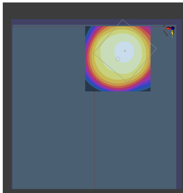
Figure 2-9 Simulated (left) and measured (right) averaged PD distribution for the following configuration: Band n260, MID Channel, Beam ID 1, H polarization, Plane B Module, plotted on the surface S2 (back) with 2mm separation distance to the camera bump.
