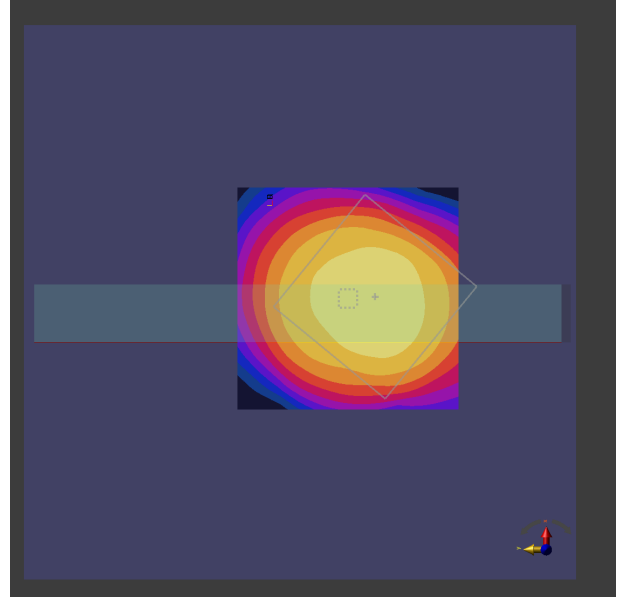
Figure 2-31 Simulated (left) and measured (right) averaged PD distribution for the following configuration: Band n258, MID Channel, Beam ID 4, H+V polarization, Plane A Module, plotted on the surface S5 (top) with 2mm separation distance to the DUT.
