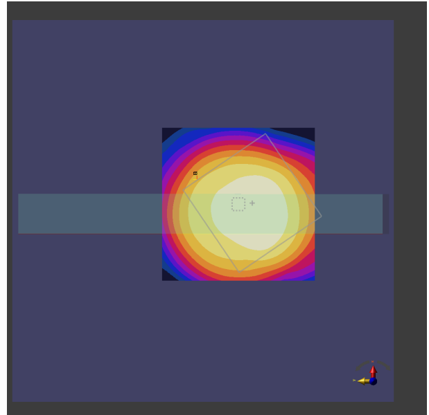
Figure 2-29 Simulated (left) and measured (right) averaged PD distribution for the following configuration: Band n258, MID Channel, Beam ID 0, V polarization, Plane A Module, plotted on the surface S5 (top) with 2mm separation distance to the DUT.
