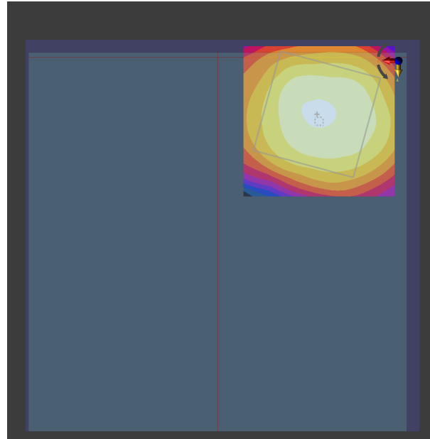
Figure 2-11 Simulated (left) and measured (right) averaged PD distribution for the following configuration: Band n260, MID Channel, Beam ID 4, V polarization, Plane B Module, plotted on the surface S2 (back) with 2mm separation distance to the camera bump.
