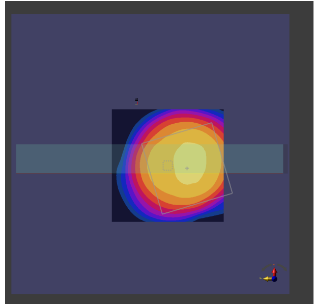
Figure 2-19 Simulated (left) and measured (right) averaged PD distribution for the following configuration: Band n261, MID Channel, Beam ID 0, H+V polarization, Plane A Module, plotted on the surface S5 (top) with 2mm separation distance to the DUT.
