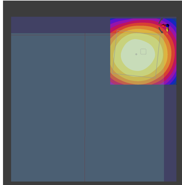
Figure 2-37 Simulated (left) and measured (right) averaged PD distribution for the following configuration: Band n258, MID Channel, Beam ID 6, H+V polarization, Plane B Module, plotted on the surface S2 (back) with 2mm separation distance to the camera bump.
