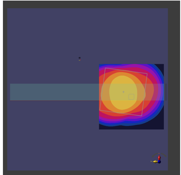
Figure 2-15 Simulated (left) and measured (right) averaged PD distribution for the following configuration: Band n261, MID Channel, Beam ID 5, H polarization, Plane A Module, plotted on the surface S5 (top) with 2mm separation distance to the DUT.
