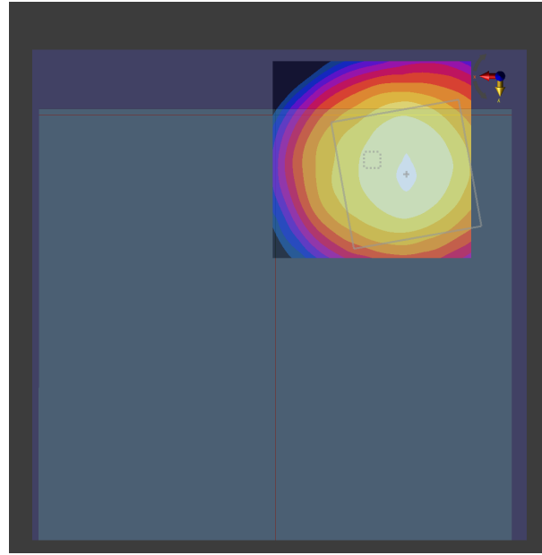
Figure 2-33 Simulated (left) and measured (right) averaged PD distribution for the following configuration: Band n258, MID Channel, Beam ID 5, H polarization, Plane B Module, plotted on the surface S2 (back) with 2mm separation distance to the camera bump.
