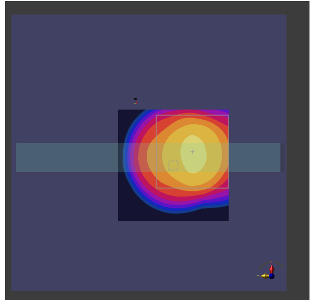
Figure 2-17 Simulated (left) and measured (right) averaged PD distribution for the following configuration: Band n261, MID Channel, Beam ID 1, V polarization, Plane A Module, plotted on the surface S5 (top) with 2mm separation distance to the DUT.
