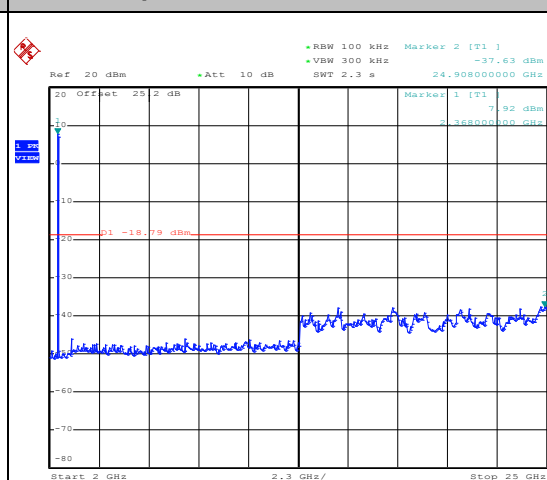
Spurious Emission 2GHz~25GHz
