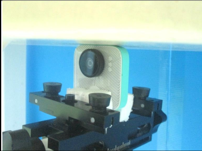
Top Side of EUT at 0 mm
