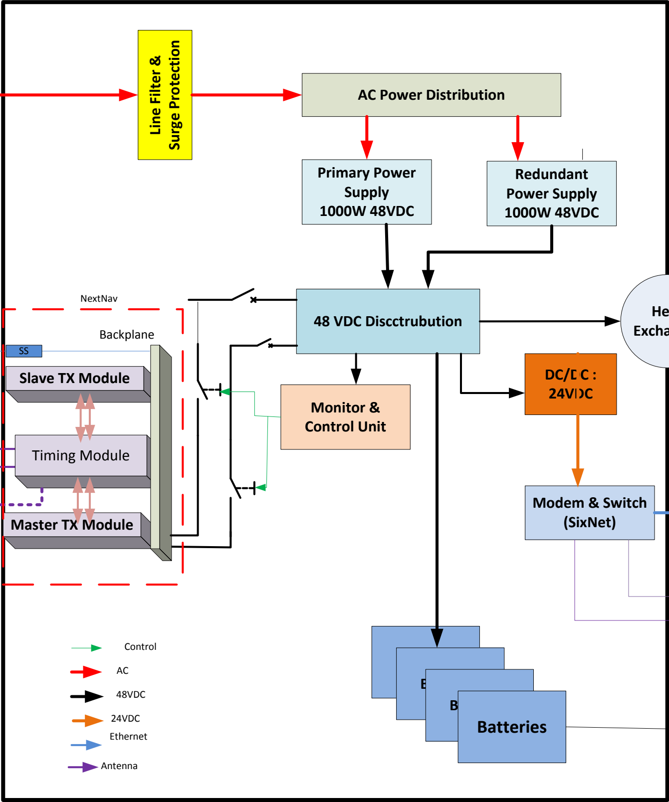
MBS System Block Diagram
