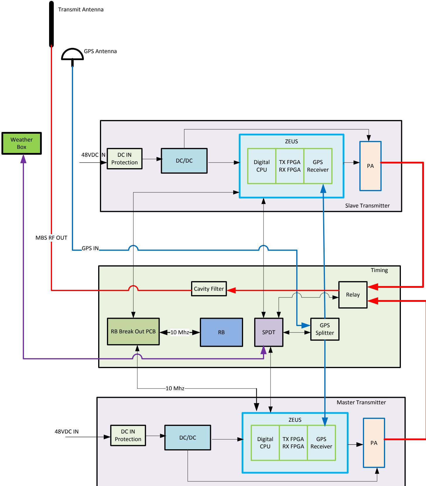
Transmitter Block Diagram
