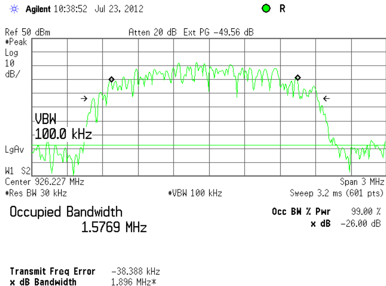
Plot 7.2.2 Occupied bandwidth test result at high frequency
