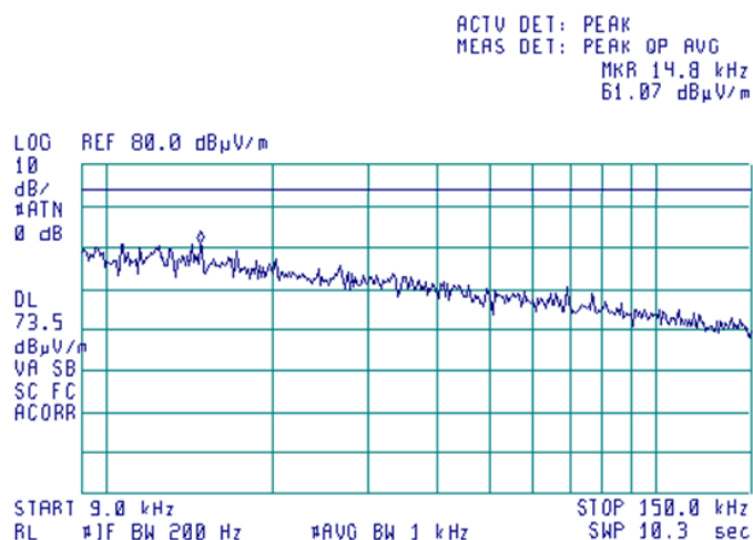
Plot 7.4.2 Radiated emission measurements in 9 - 150 kHz range
