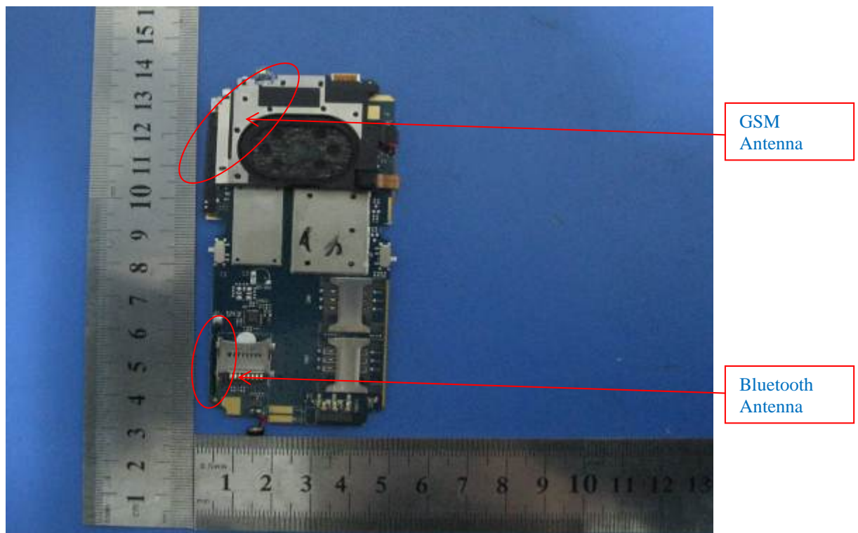
Antenna - Front View
