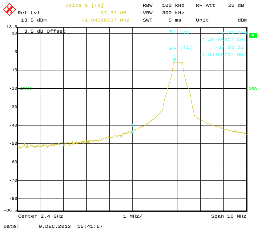
BDR (GFSK): Band Edge-Left Side
