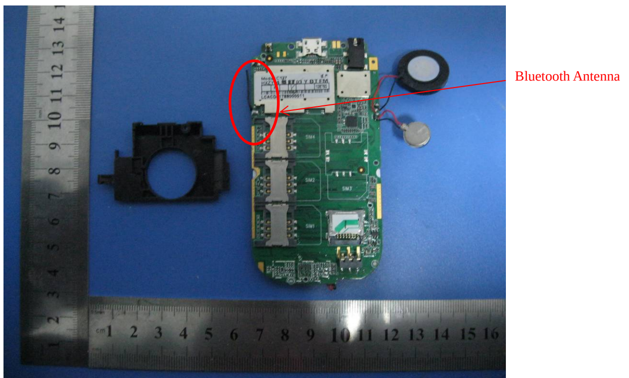
Bluetooth Antenna - Top View
