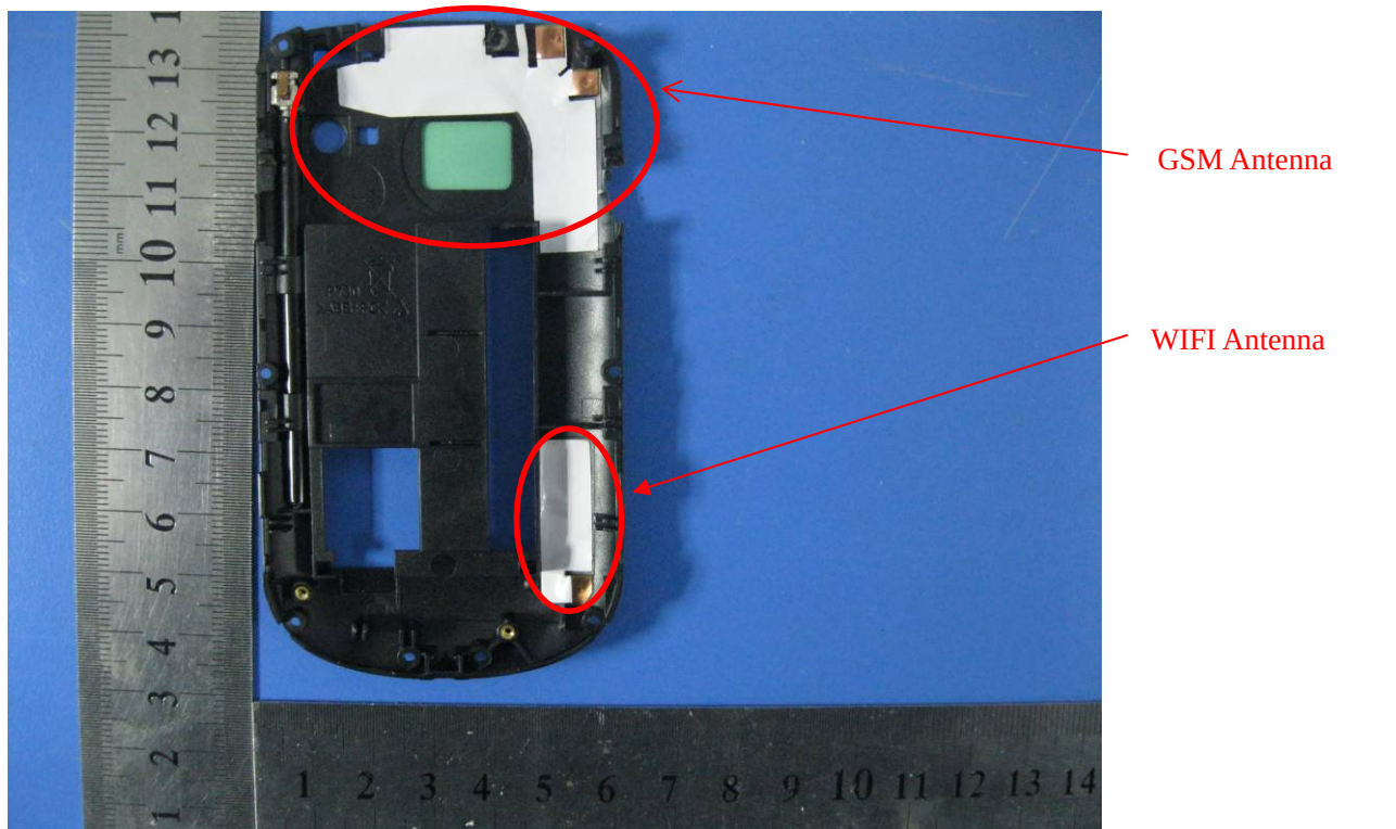
GSM Antenna - Top View
