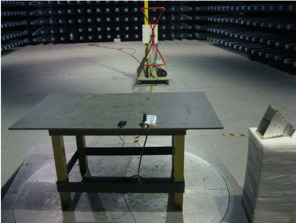
Above 1GHz: Radiated Emissions
