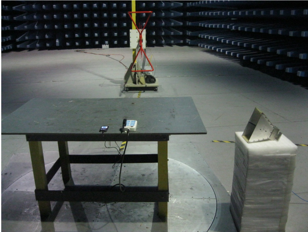
Front View of Radiated Emissions below 1GHz
