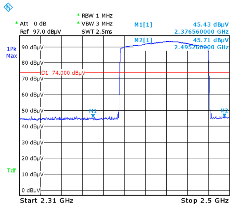
8DPSK hopping-PK
