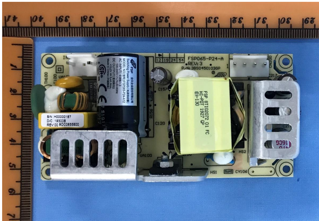
Internal photo, PSU FSP065-24P-A12 PCBA side
