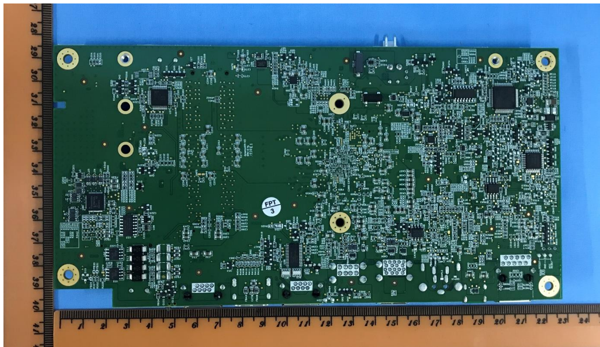
Mainboard – PCB trace
