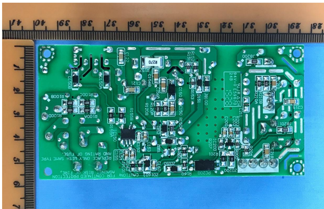
Internal photo, PSU PCB trace
