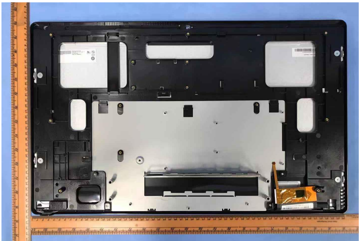
LCD panel
