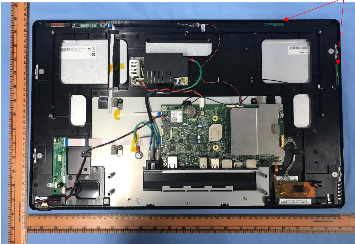
Back cover removed
