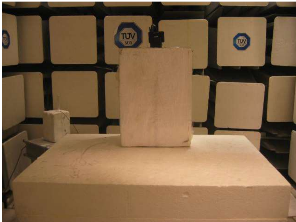
Out of Band Emissions (Radiated) Test Setup (Front View)
