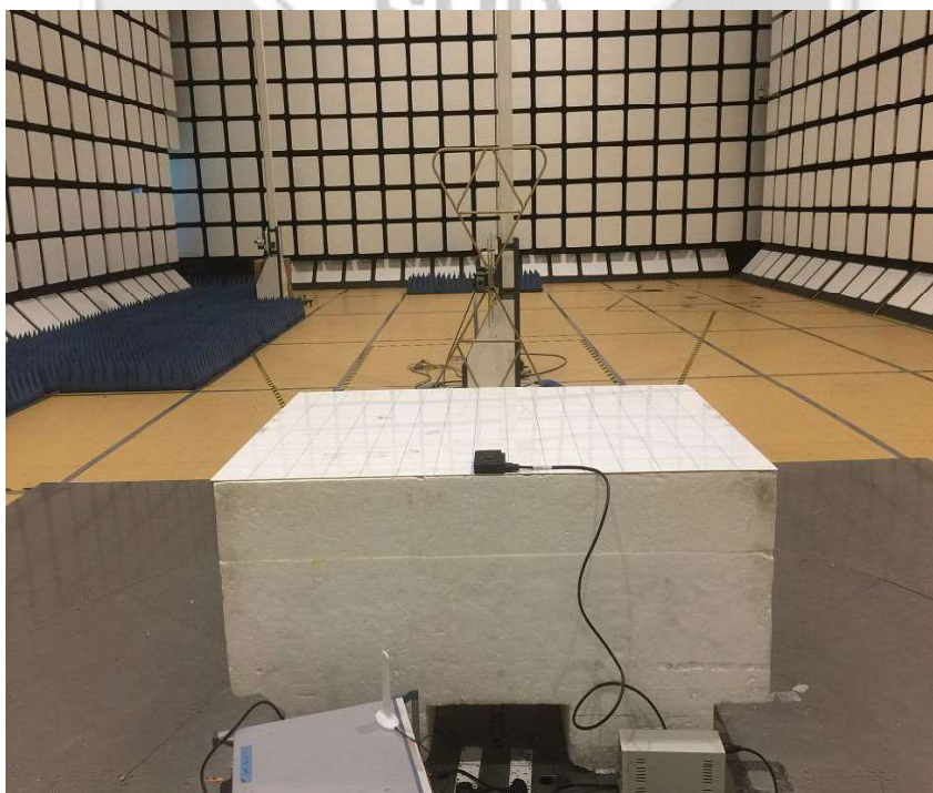
Receiver Spurious Emissions Test Setup (Rear View)
