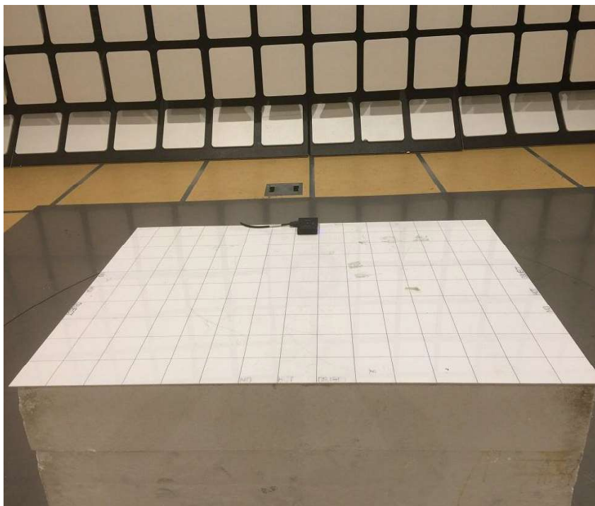
Receiver Spurious Emissions Test Setup (Front View)
