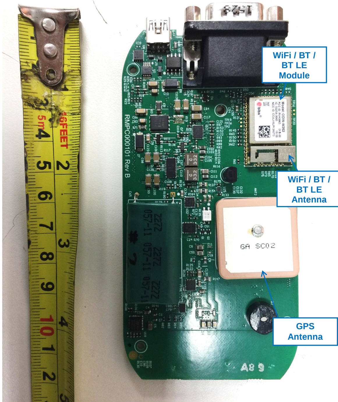
Main-Board PCB Trace Side
